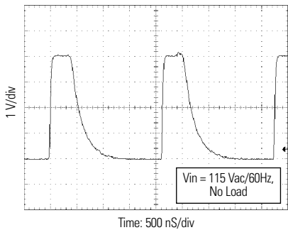
19. Free-running Sync Output
