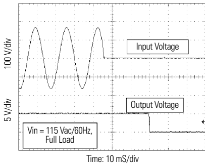
16. Input Voltage Turn-Off vs. Output Voltage
