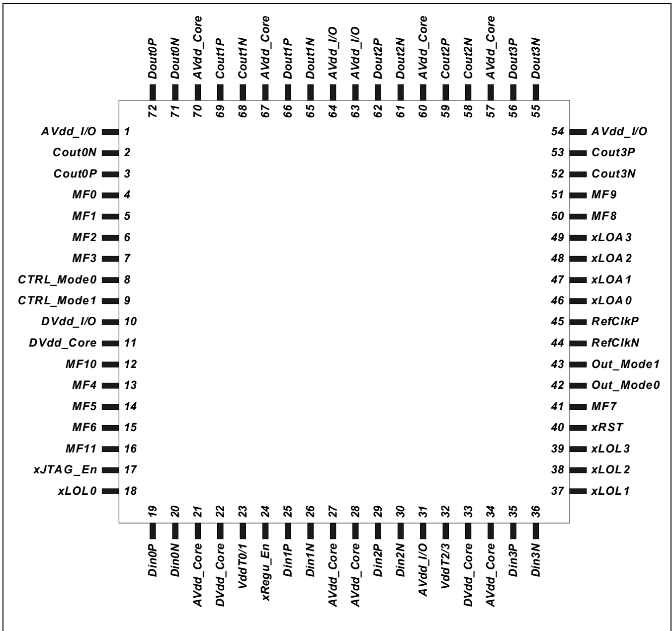
Figure 1-11. M2125x Pinout Diagram (Top View)
