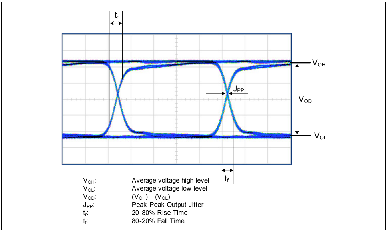
Figure 2-2. Definitions of Eye Parameters
