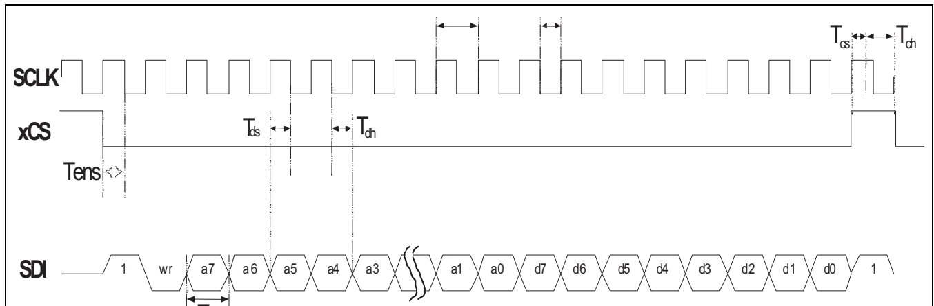
Figure 1-5. Serial WRITE Mode
