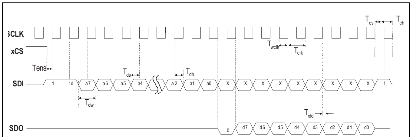
Figure 1-6. Serial READ Mode
