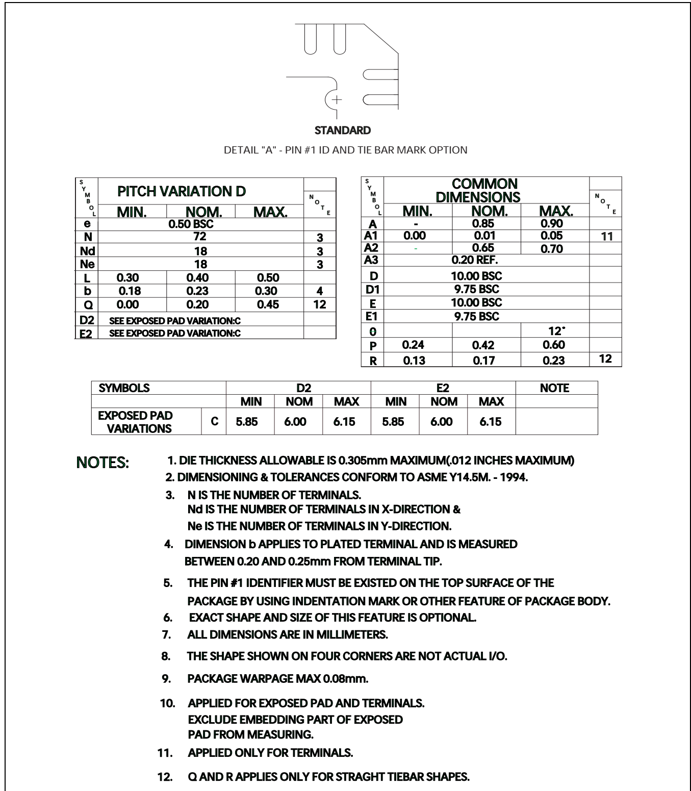
Figure 2-11. 72-Pin Package Dimensions
