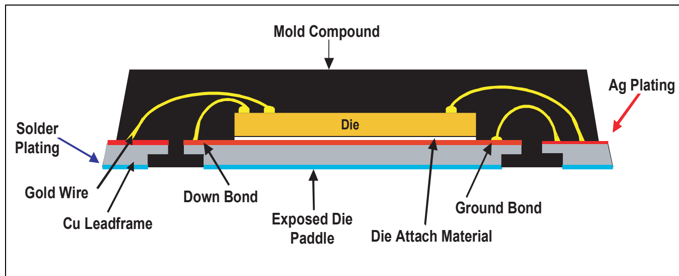
Figure 2-8. Cross-Section of QFN Package
