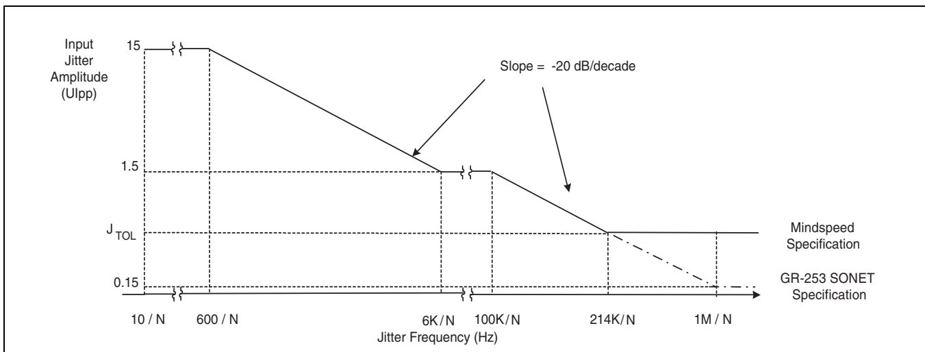
Figure 2-6. SONET Jitter Tolerance Specification Mask
