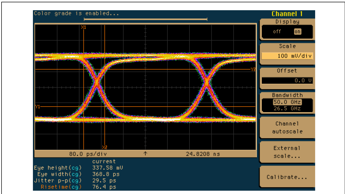
Figure 1-8. STS-48 waveform at M21250 output with input shown in Figure 1-7
