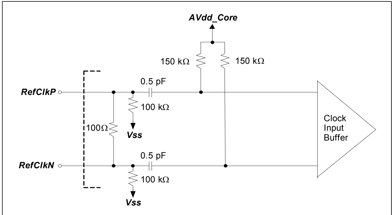
Figure 2-3. Reference Clock Input Internal Circuitry
