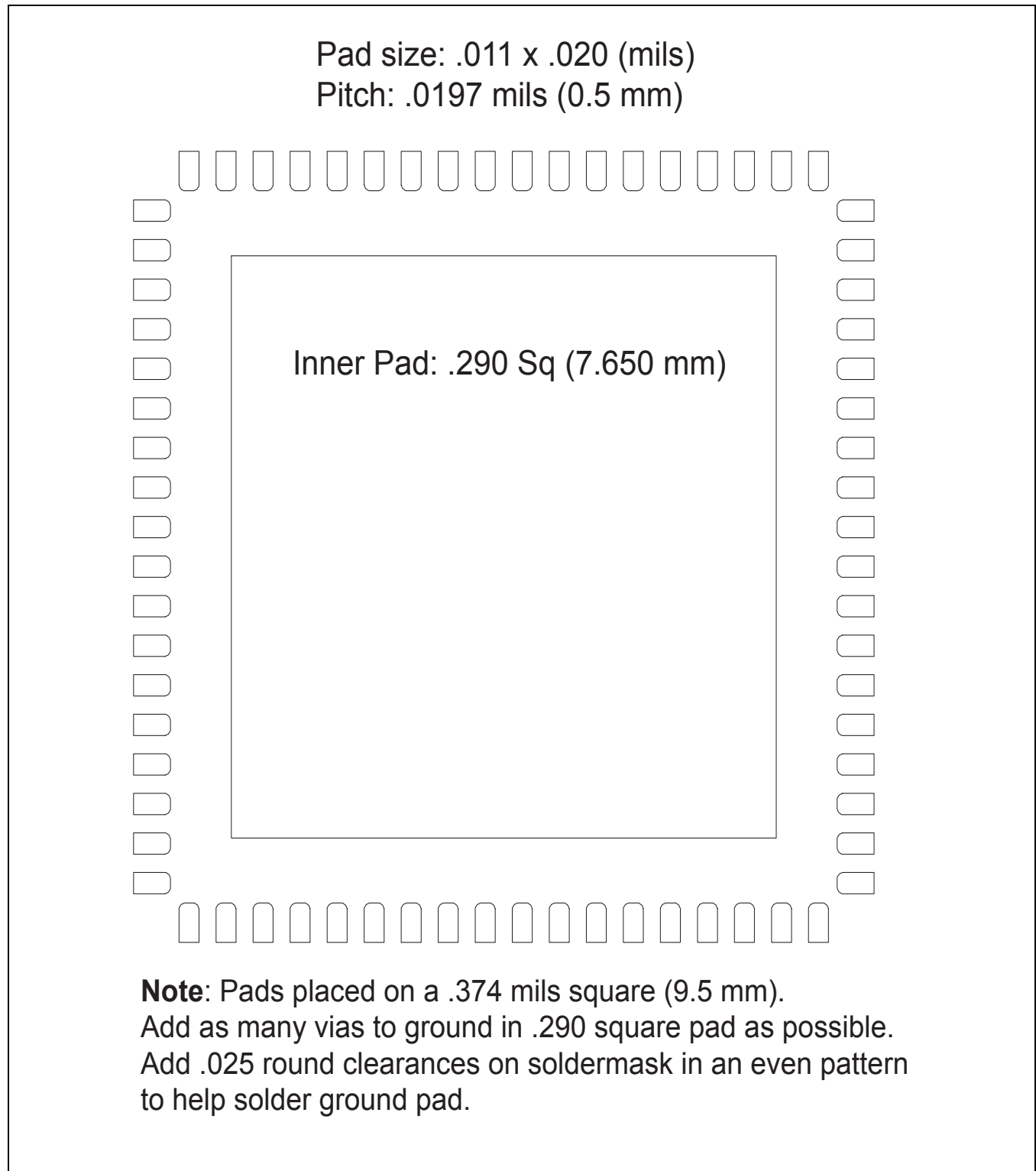
Figure 2-12. PCB Footprint for 72-Pin 10 mm QFN Package
