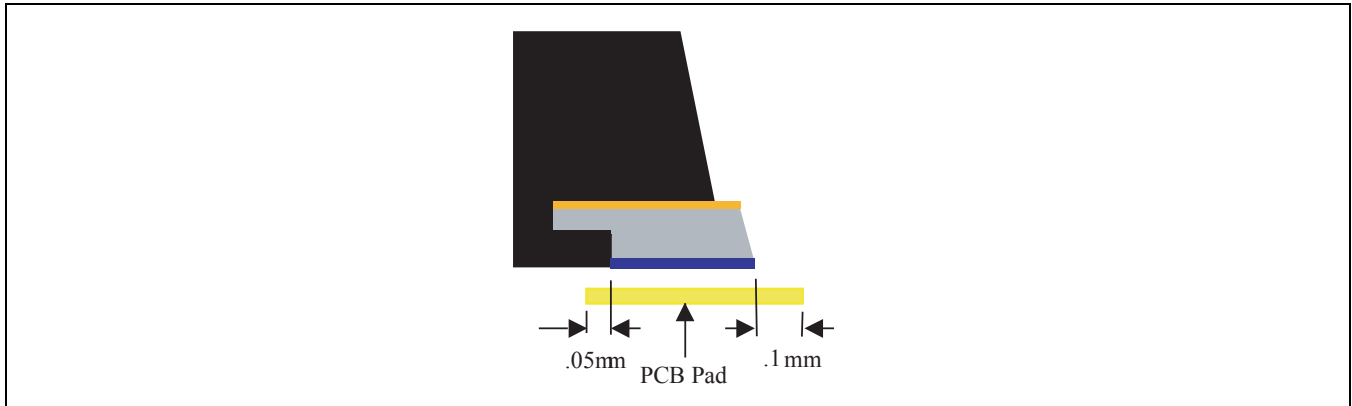
Figure 2-13. PCB Pad Extensions
