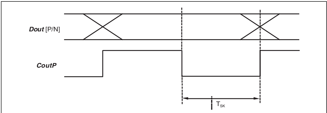
Figure 2-4. Clock and Data Output Skew Timing
