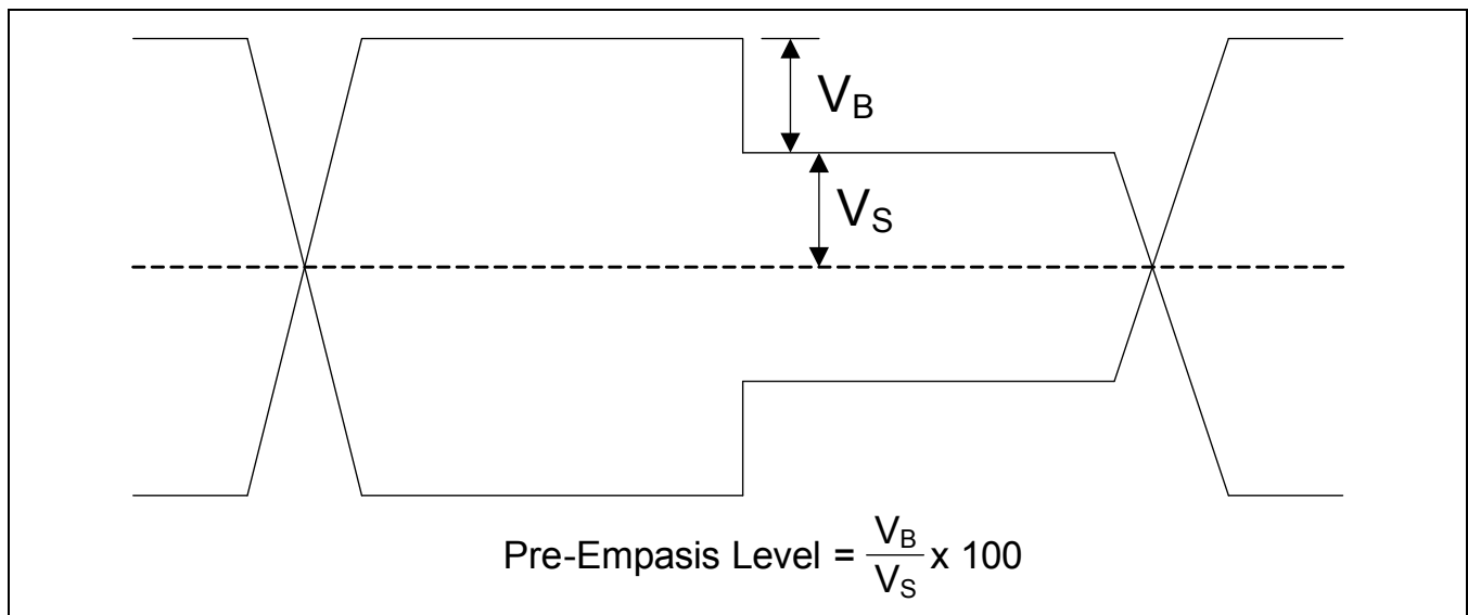
Figure 1-9. Definition of Pre-Emphasis Levels
