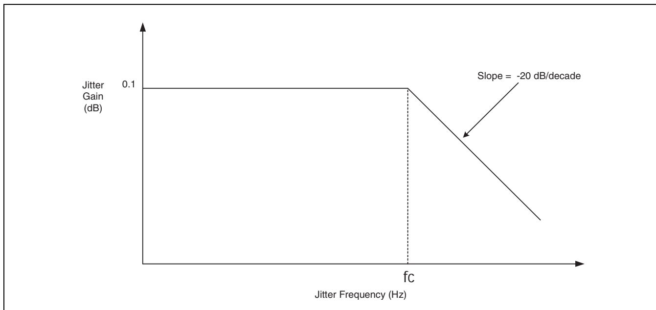
Figure 2-7. SONET/SMPTE Jitter Transfer Specification Mask
