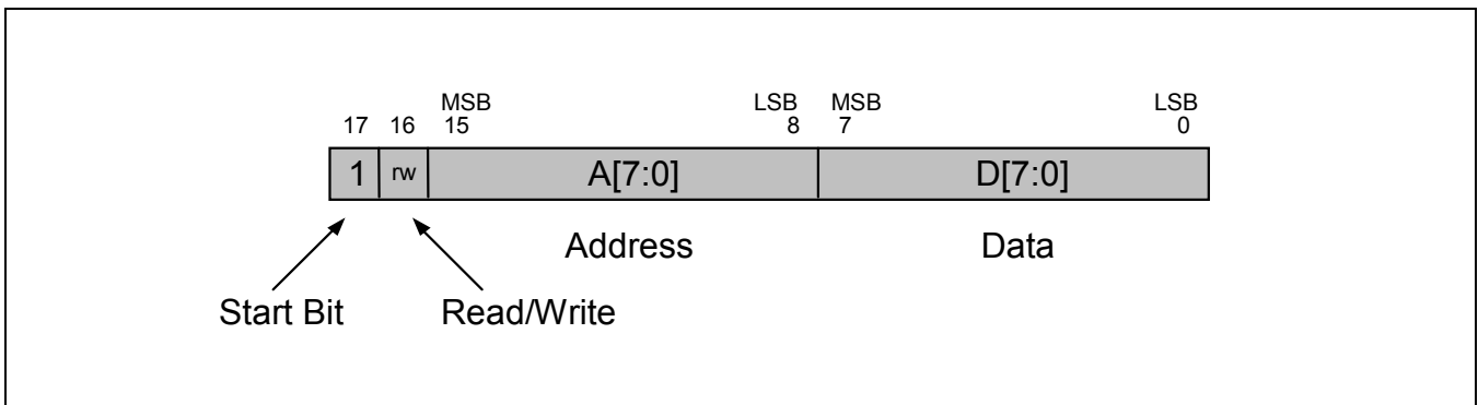
Figure 1-4. Serial Word Format
