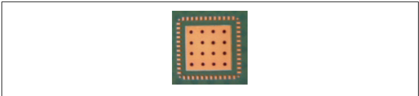
Figure 2-14. Recommended Via Array for Thermal Pad
