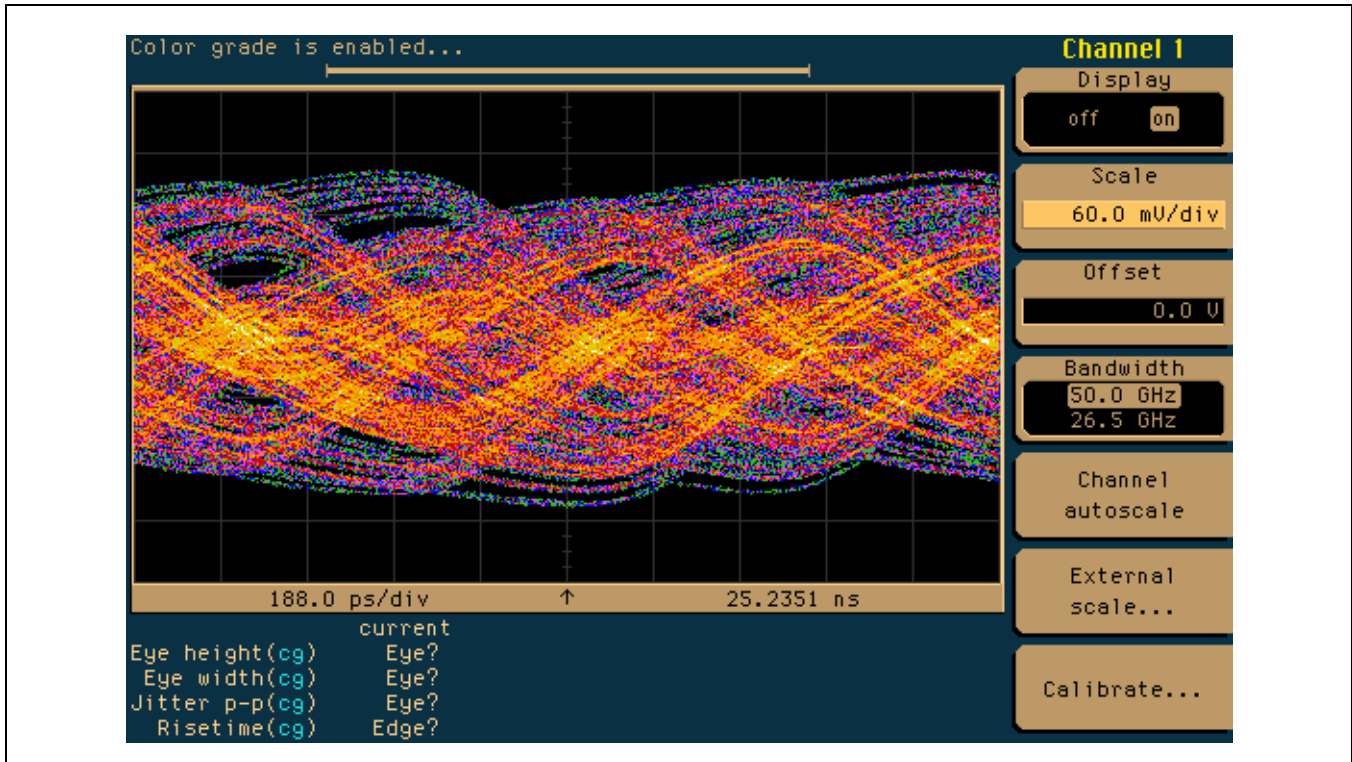
Figure 1-7. STS-48 waveform after transmission through 76" of PCB traces (input to M21250)
