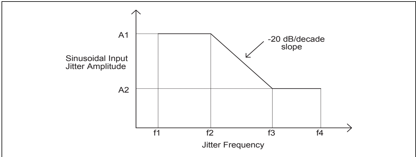
Figure 2-5. SMPTE Jitter Tolerance Specification Mask
