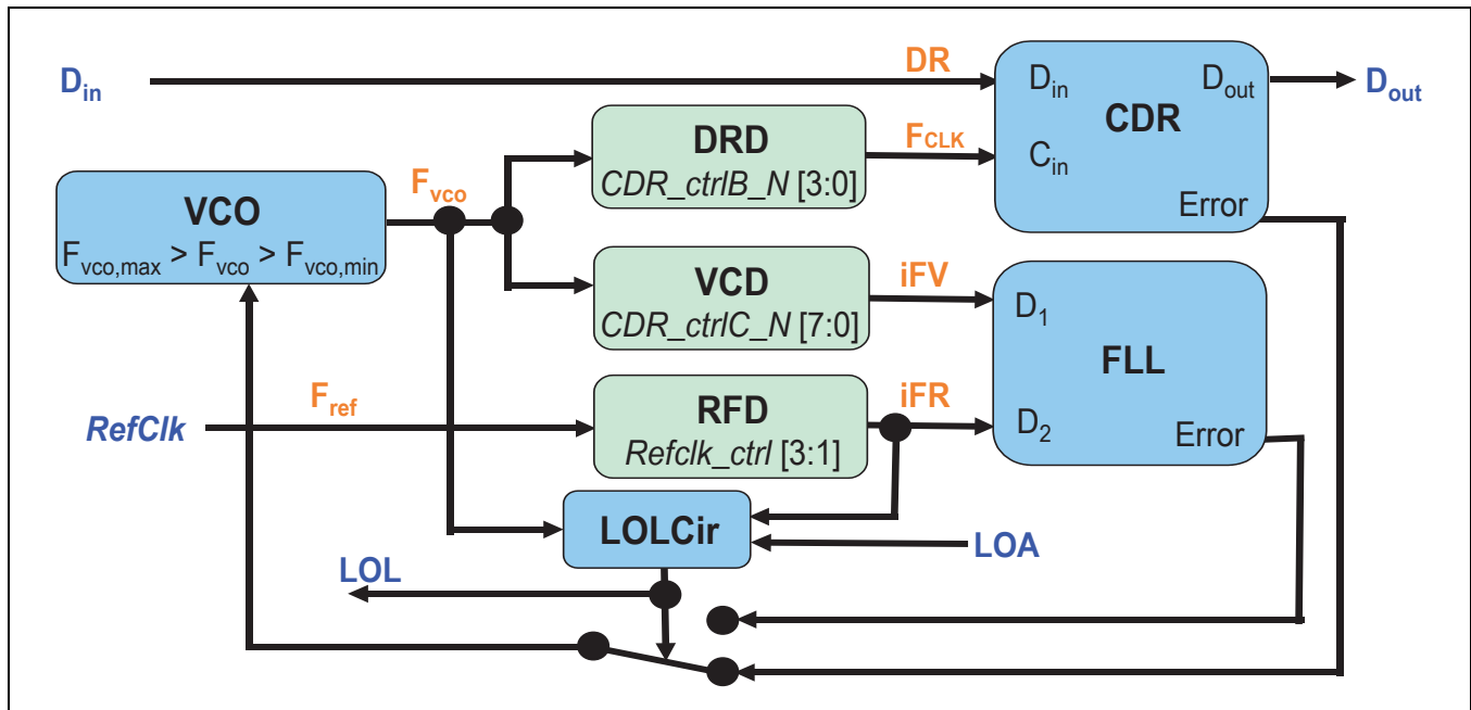
Figure 1-10. Block Diagram of Frequency Acquisition Circuits
