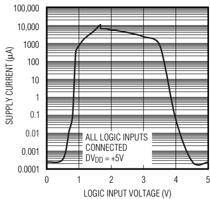
DVDD SUPPLY CURRENT vs. LOGIC INPUT VOLTAGE
