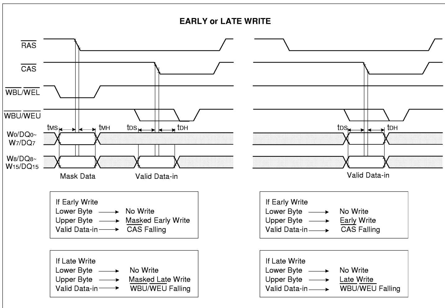
Figure 3. Byte Write and New Masked Write Cycle Example2.
