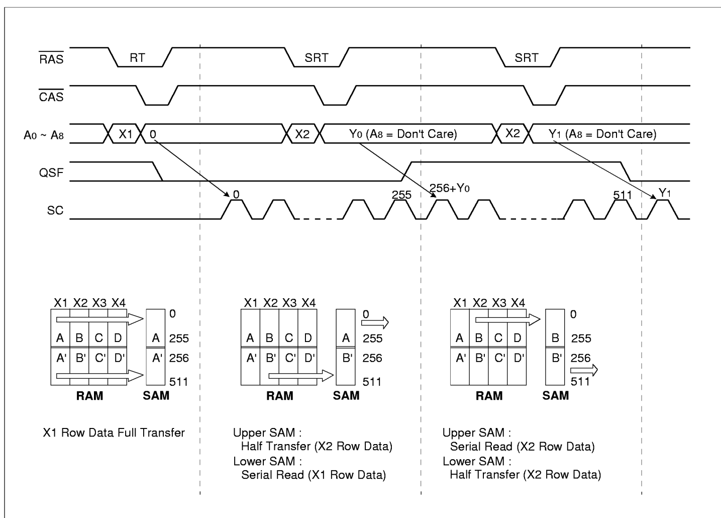
Figure 7. Split Read Transfer Normal Usage
