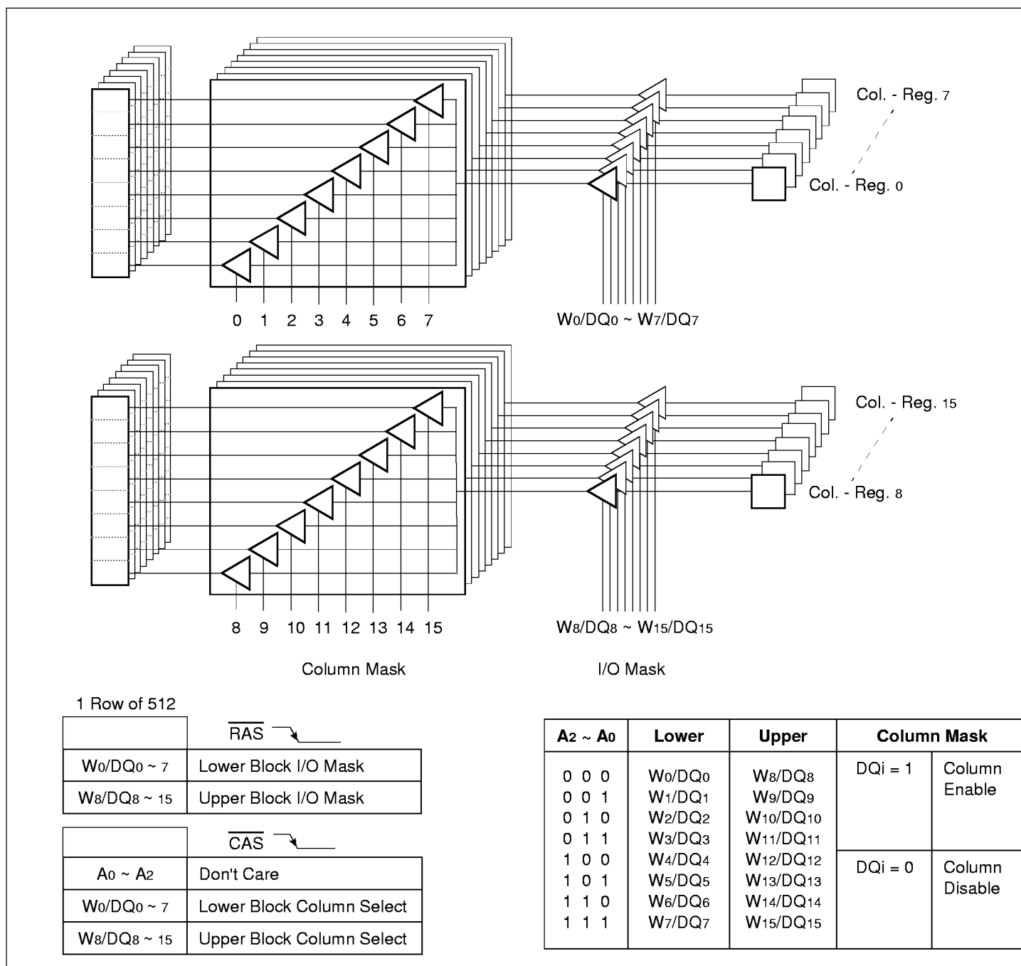
Figure 5. Block Write Scheme
