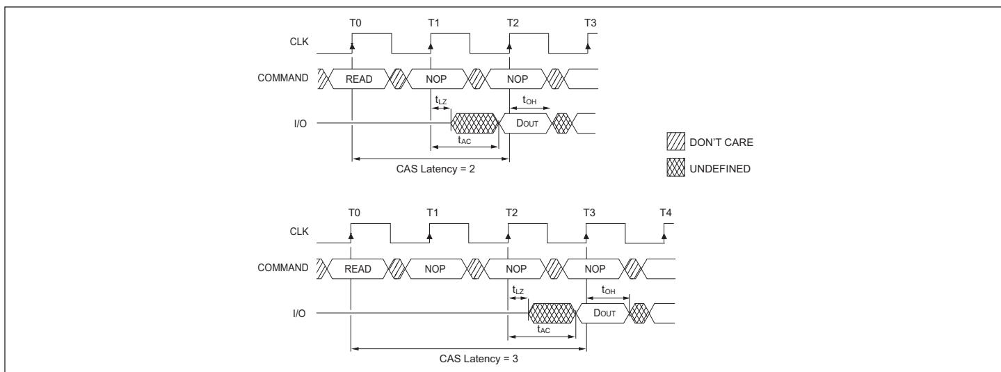
FIGURE 4 – CAS LATENCY
