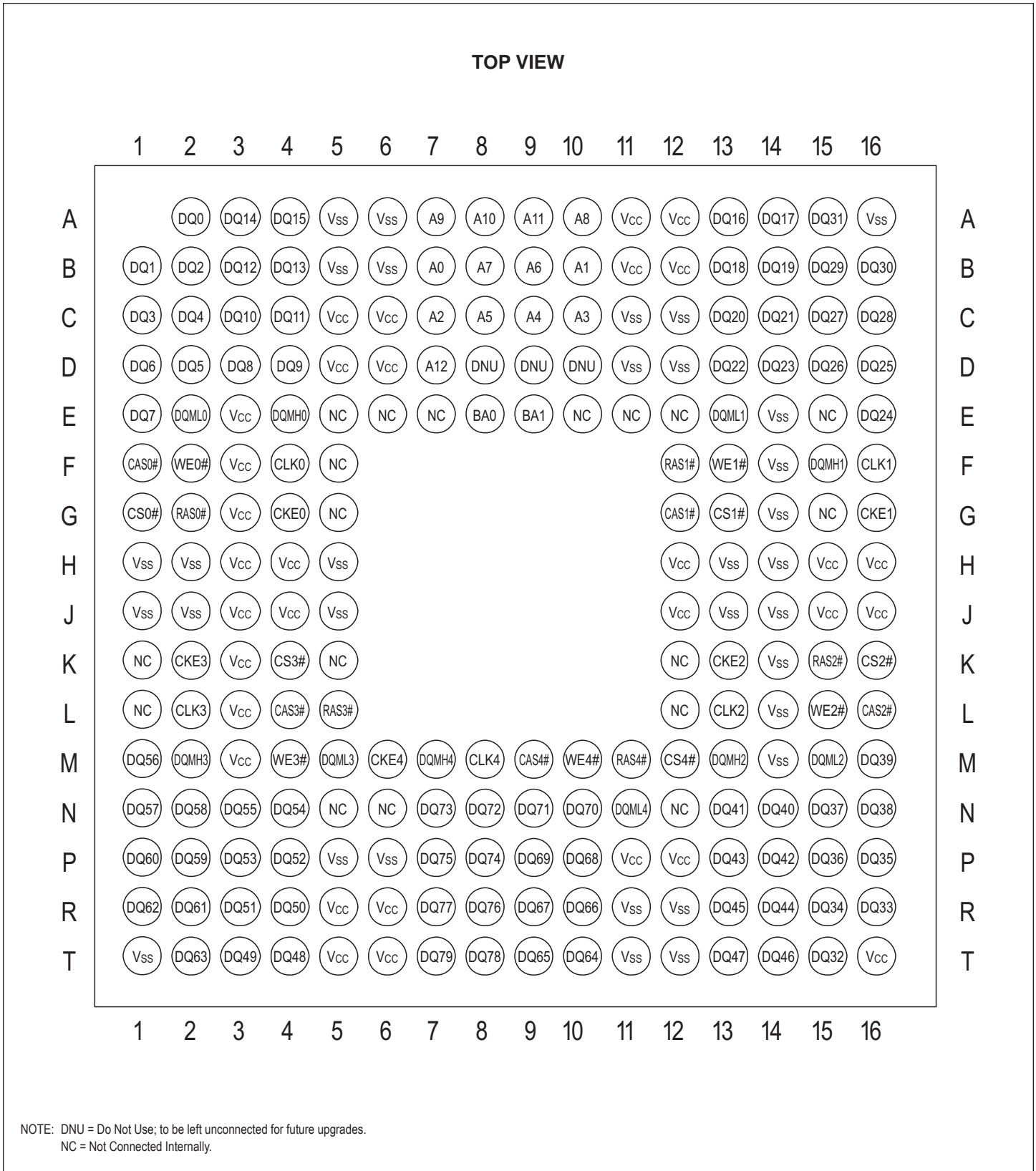
FIGURE 1 – PIN CONFIGURATION
