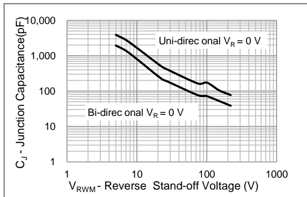
Fig.4 Typical Capacitance
