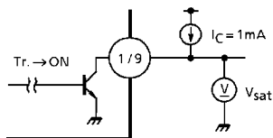
V sat① , V sat⑨ Test Circuit
