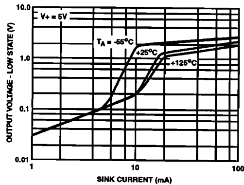
FIGURE 4. OUTPUT VOLTAGE LOW STATE vs SINK CURRENT AT V_+ = 5\text{V}
