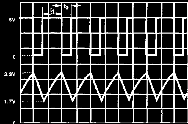
FIGURE 14. TYPICAL WAVEFORMS FOR REPEAT CYCLE TIMER
