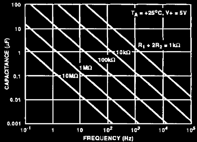
FIGURE 15. FREE RUNNING FREQUENCY OF REPEAT CYCLE TIMER WITH VARIATION IN CAPACITANCE AND RESISTANCE
