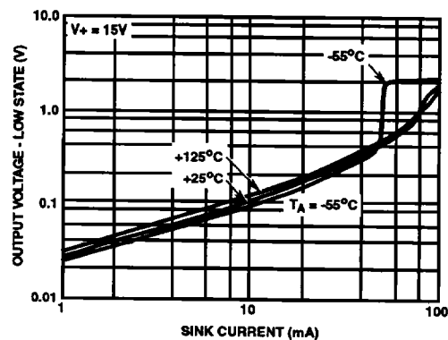
FIGURE 6. OUTPUT VOLTAGE LOW STATE vs SINK CURRENT AT V_+ = 15\text{V}
