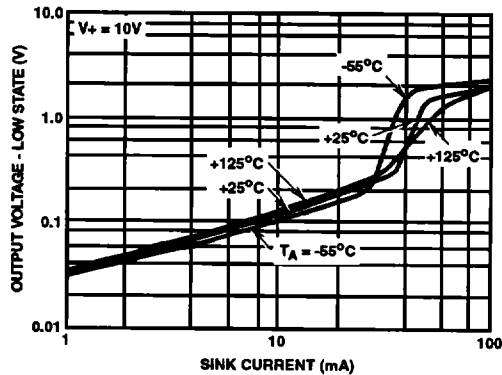
FIGURE 5. OUTPUT VOLTAGE LOW STATE vs SINK CURRENT AT V_+ = 10\text{V}
