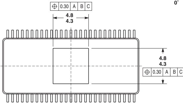
VIEW C-C
