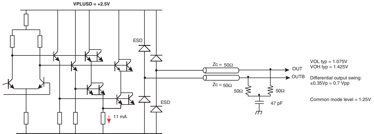
Figure 8-7. 50Ω Terminated Differential Outputs
