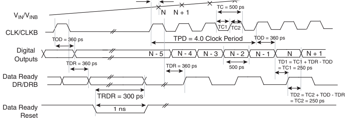
Figure 8-1. EV10AS008B Timing Diagram (2 Gbps Clock Rate) Data Ready Reset, Clock Held at Low Level
