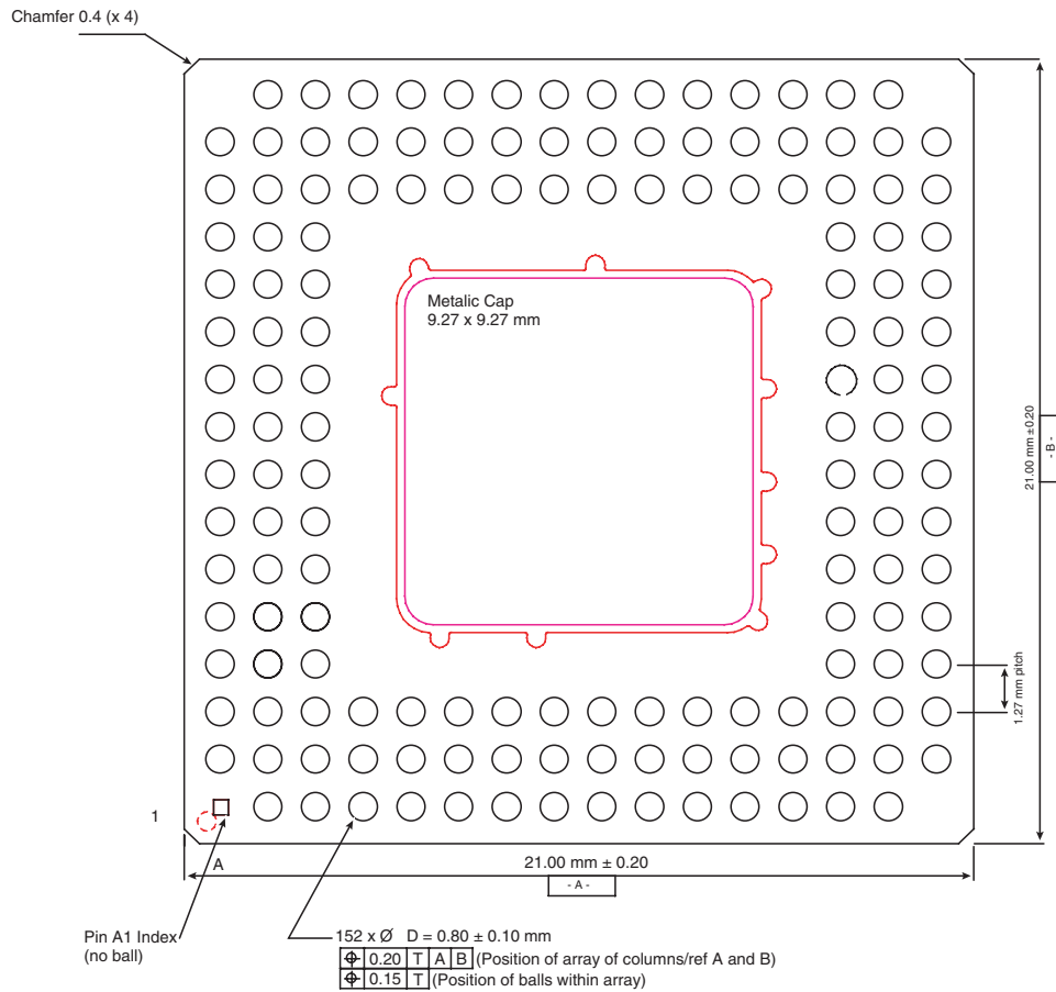
Figure 4-2. Mechanical Description Bottom View
