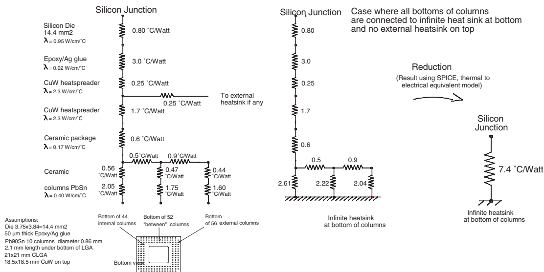
Figure 5-3. Thermal Net
