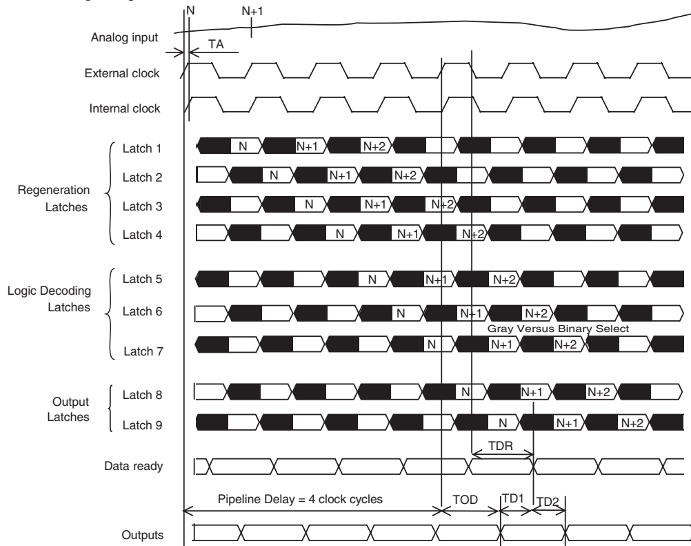
Figure 3-1. Timing Diagram
