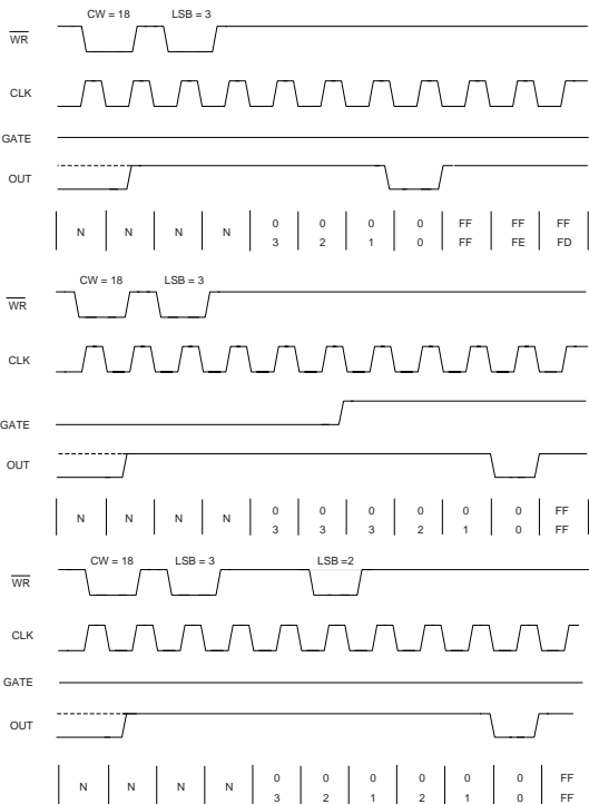
Figure 2-16: Mode 4 Timing
