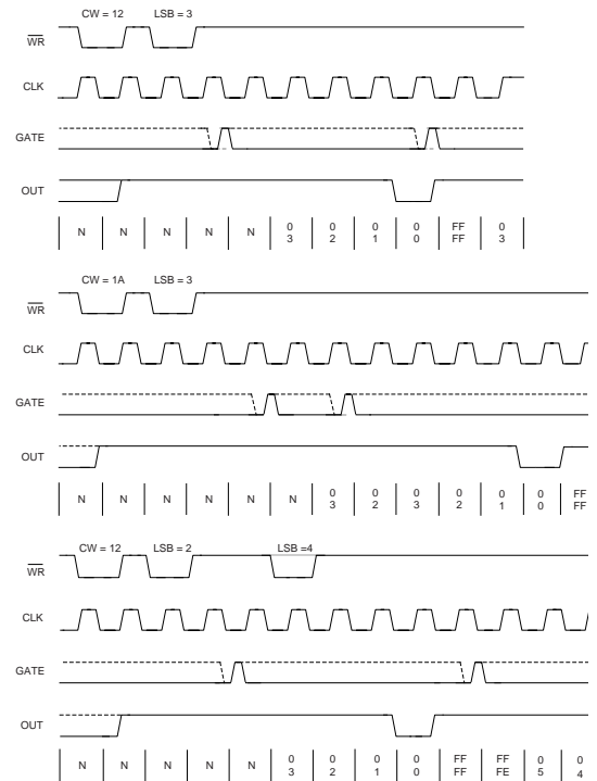
Figure 2-17: Mode 5 Timing
