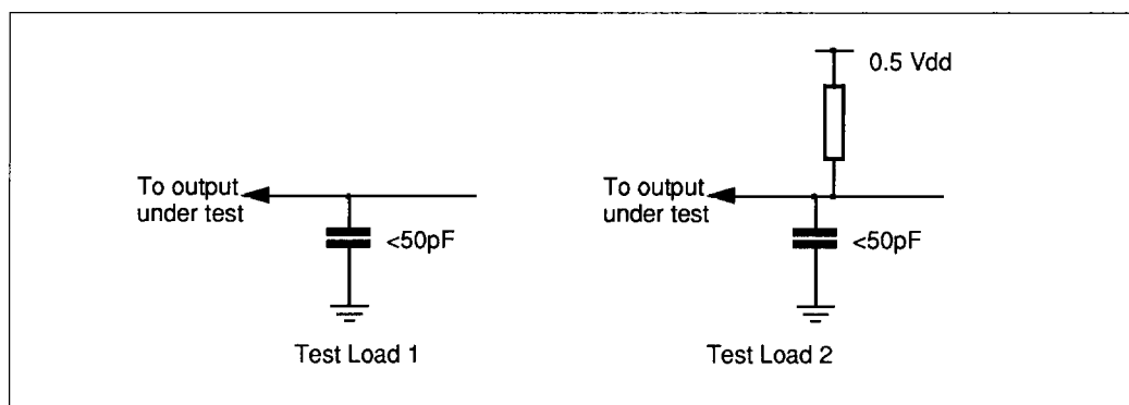
Figure 31b : Output Loads for AC measurements
