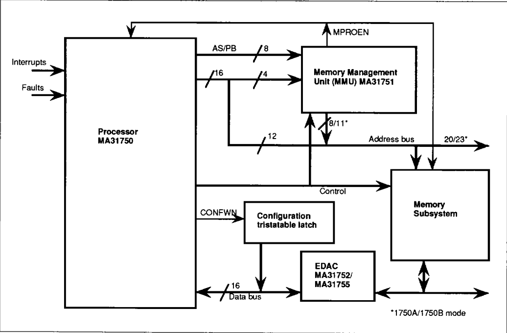
Figure 32: Typical Small System Configuration
