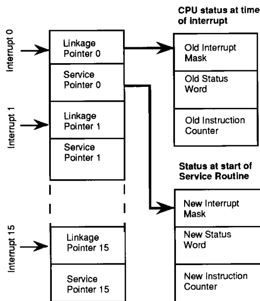
Figure 11: Interrupt Vectoring
