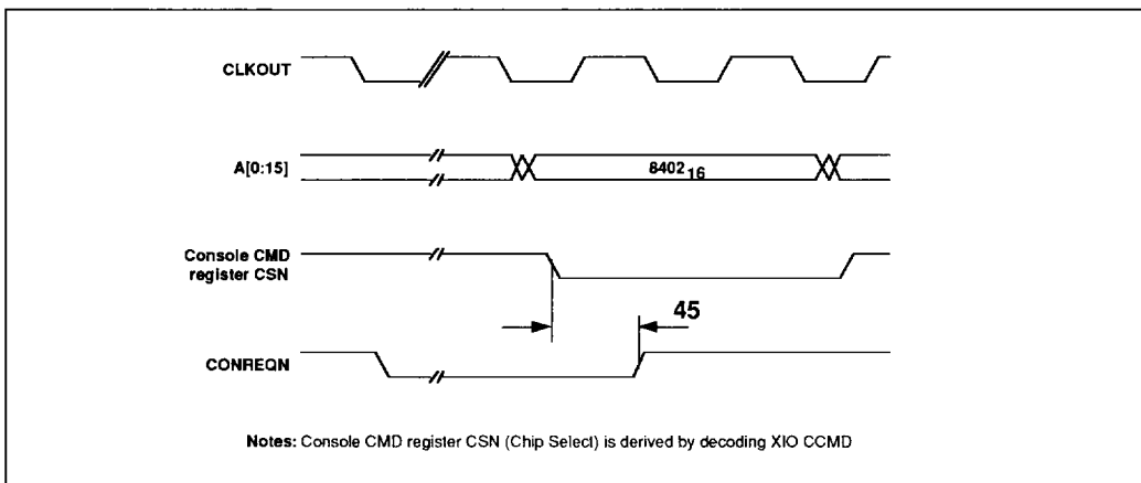
Figure 30: Console Request Timings
