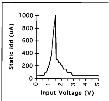
Figure 37: Input Characteristic
