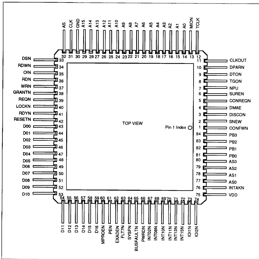
Figure 39a: 84-Lead Flatpack - Package Style F
