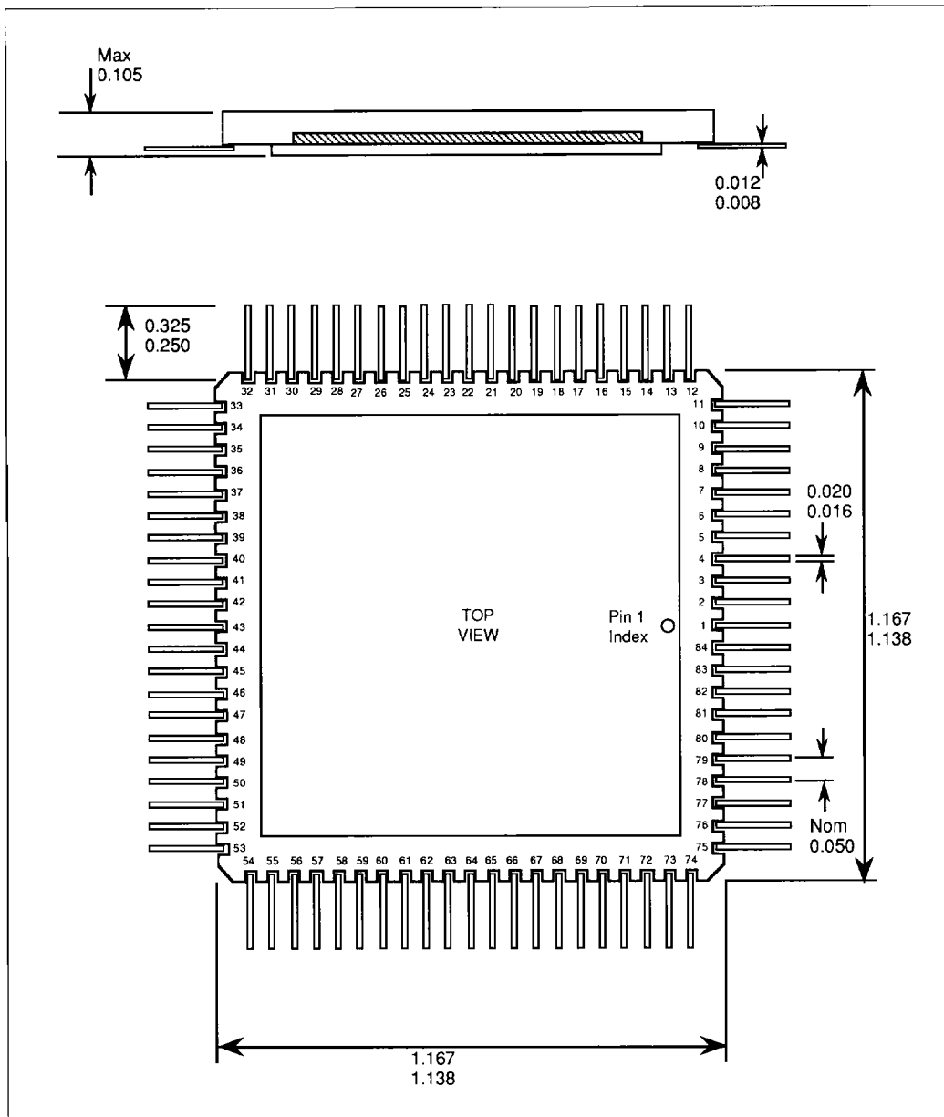
Figure 39b: 84-Lead Flatpack - Package Style F
