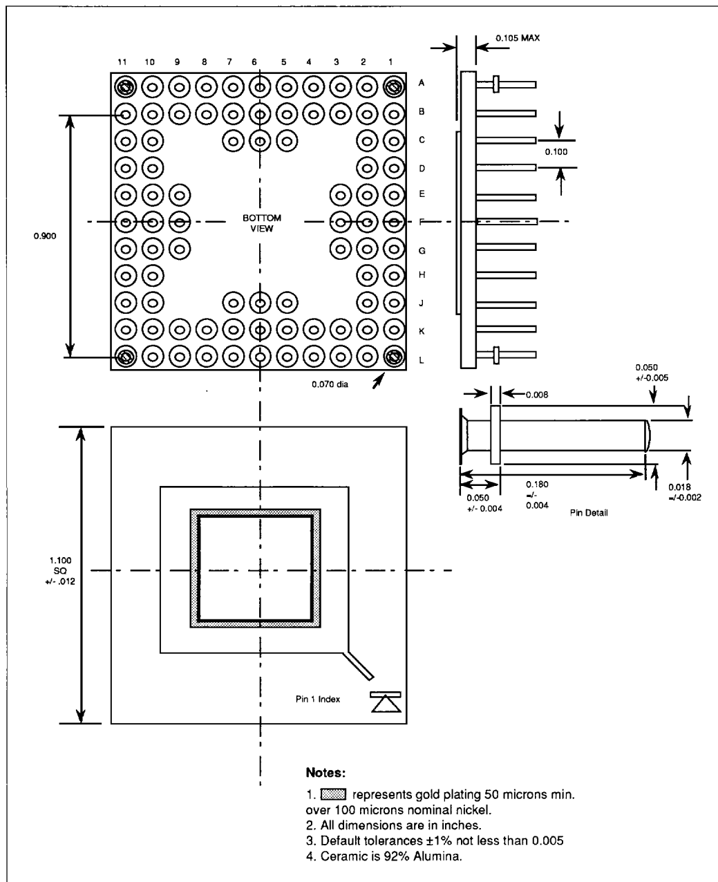
Figure 40b: 84-Pin Grid Array - Package Style A
