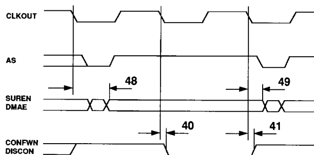
Figure 28: DPARN Input Timing
