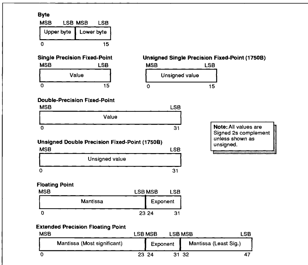
Figure 16: Data Formats
