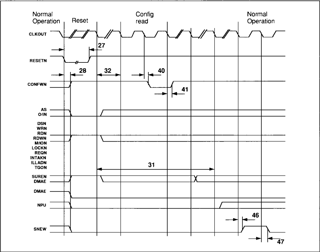
Figure 25: Reset Timing
