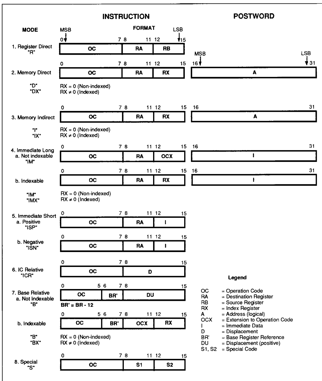
Figure 18: Addressing Modes
