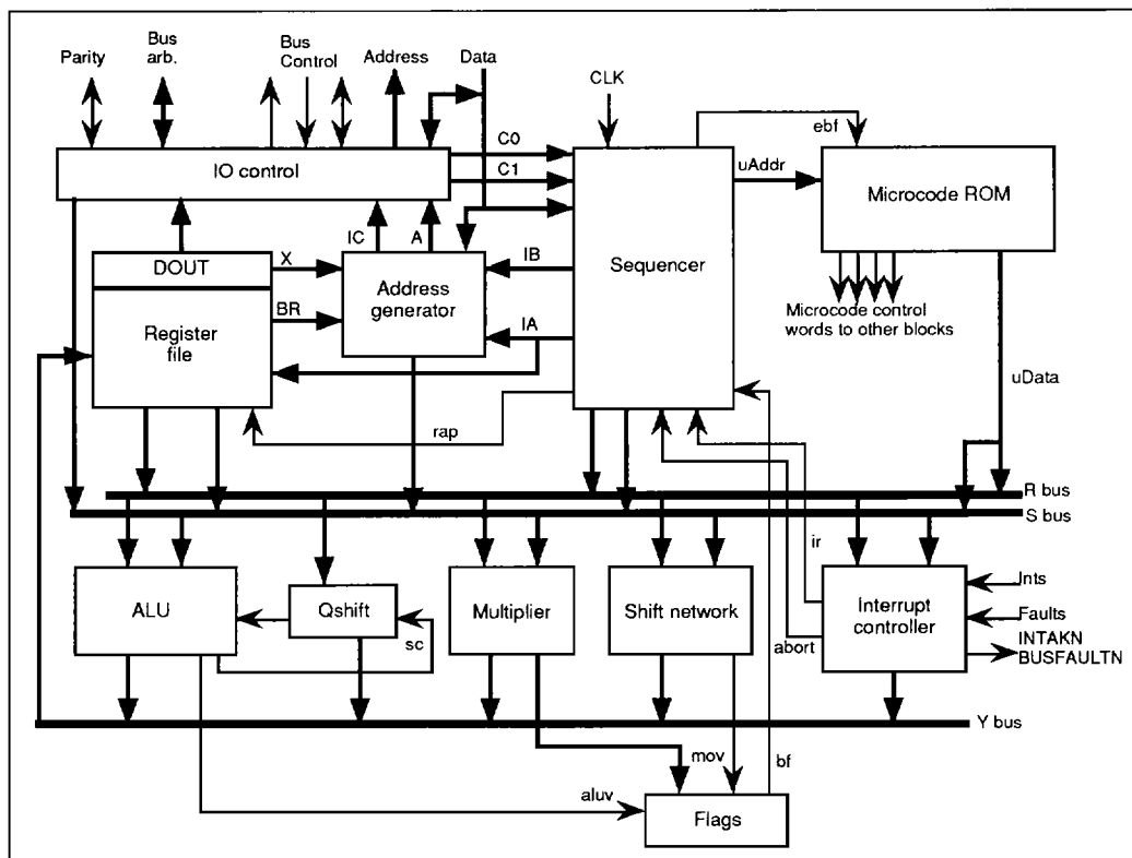
Figure 1: Architecture
