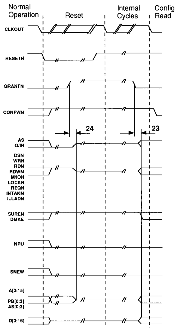
Figure 26: GRANTN during RESETN Low
