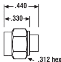
3201-1A-9 SMA Straight Male Semi-Rigid/ Ultra-Flex-
