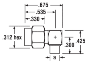
3221-1A-1 SMA Right Angle Male Semi-Rigid/ Ultra-Flex-
