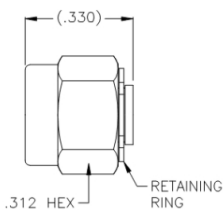
3136-9 SMA Straight Male Semi-Rigid/ Ultra-Flex-Solder
