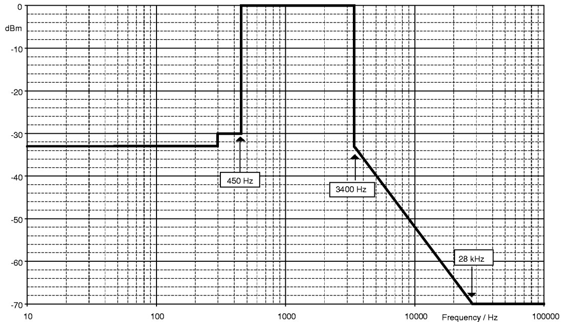
Figure 6: Tx limits at 1200bps rate
