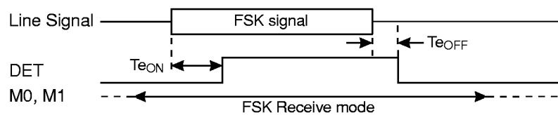
Figure 4: FSK Level Detector Operation
