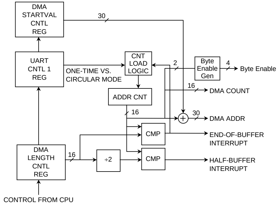
Figure 16.2.1 UART DMA
