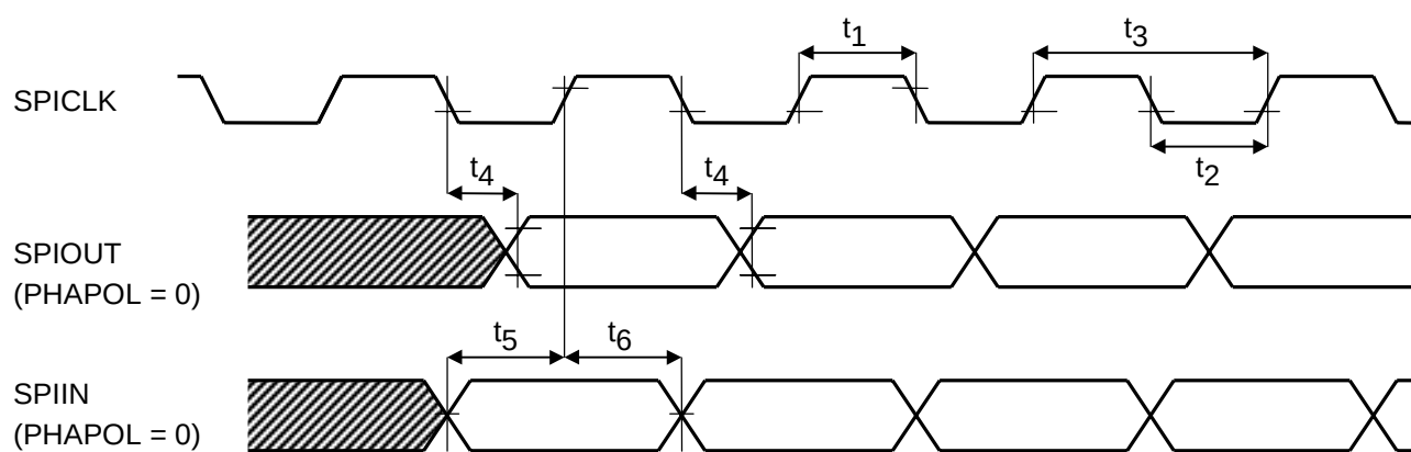
SPI Timing
