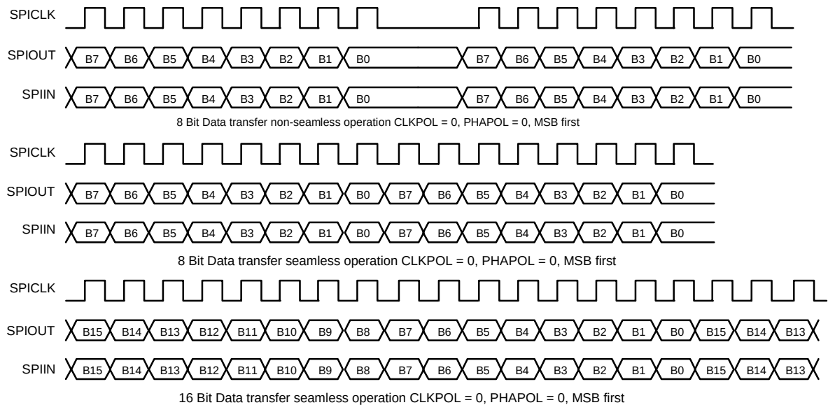
Figure 14.2.2 SPI Timing
