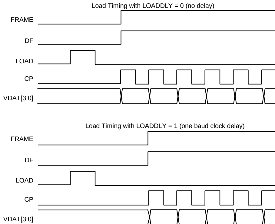
Figure 17.3.2 LOADDLY Timing
