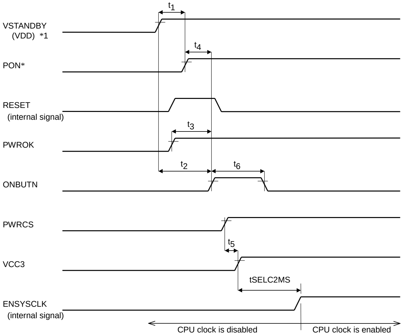
Power Timing
