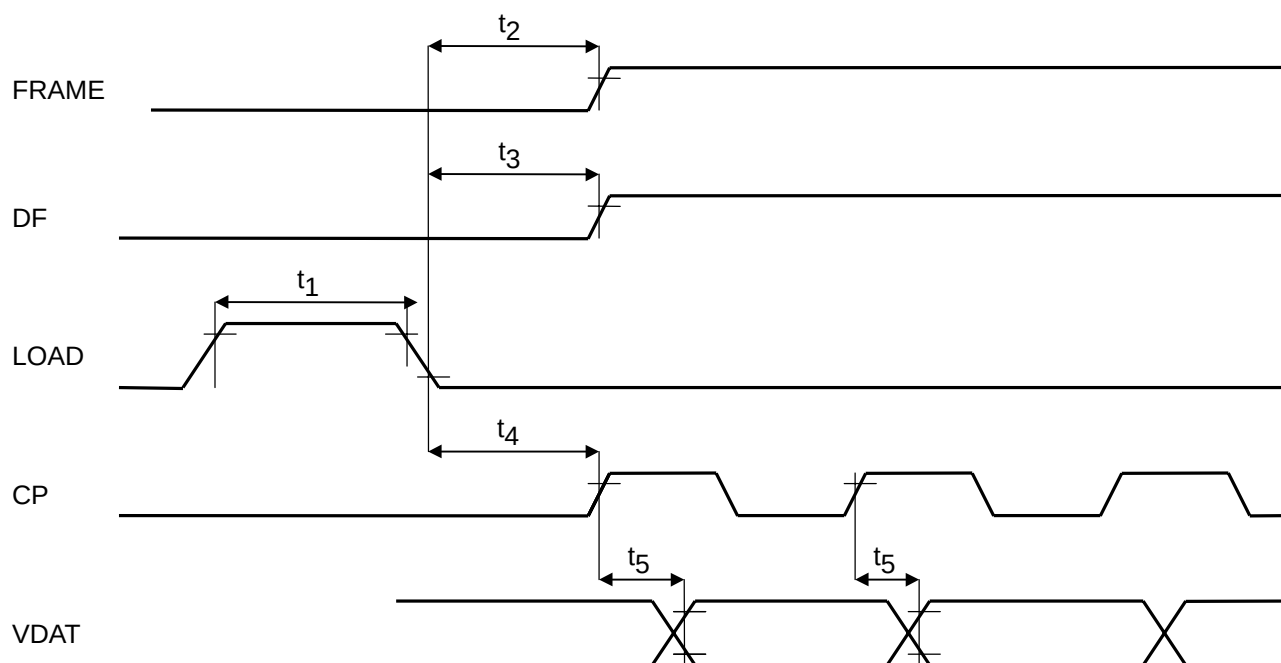
VIDEO Timing
