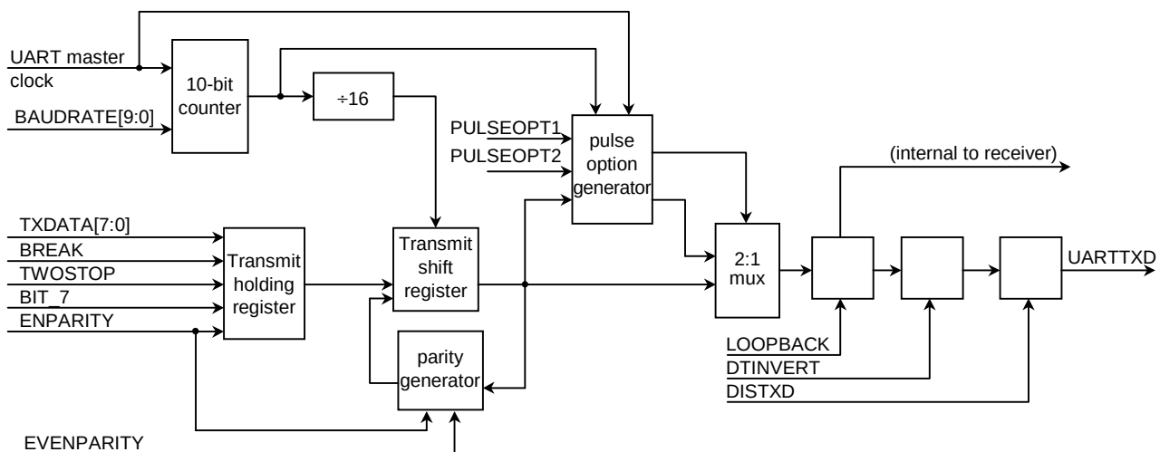
Figure 16.3.1 UART Transmitter
