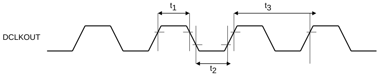
DCLKOUT Timing
