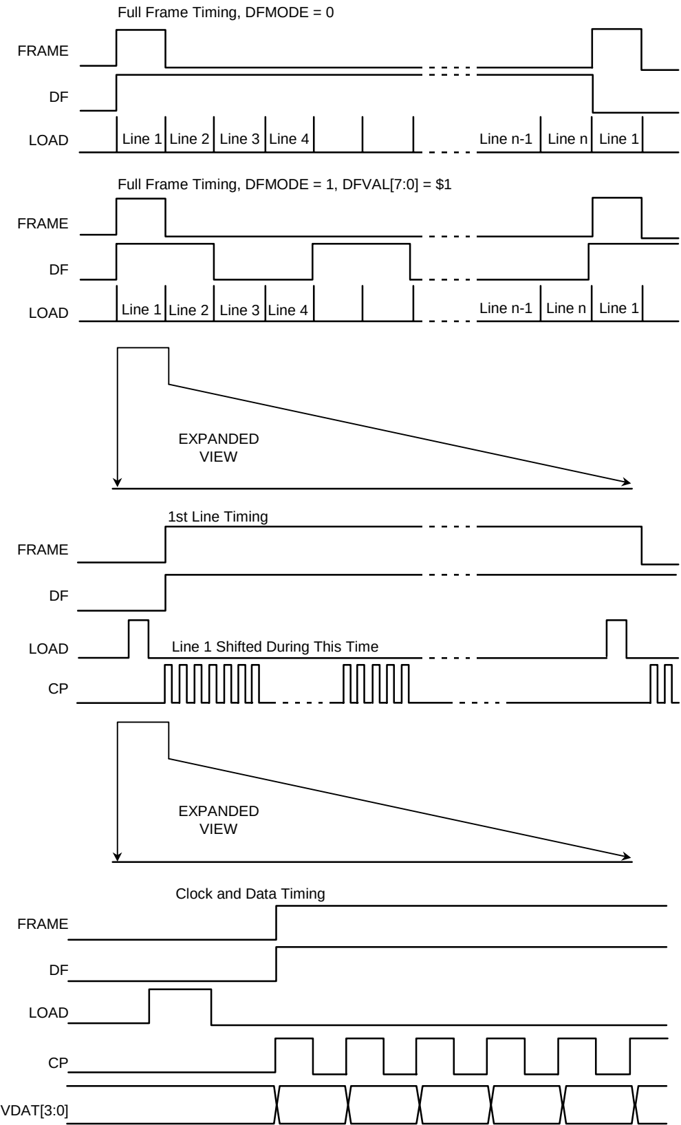
Figure 17.2.3 LCD Timing
