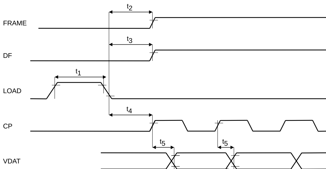
VIDEO Timing
