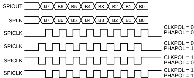
Figure 14.2.3 CLKPOL/PHAPOL Timing
