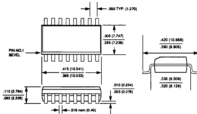
Figure 6 Package Dimensions
