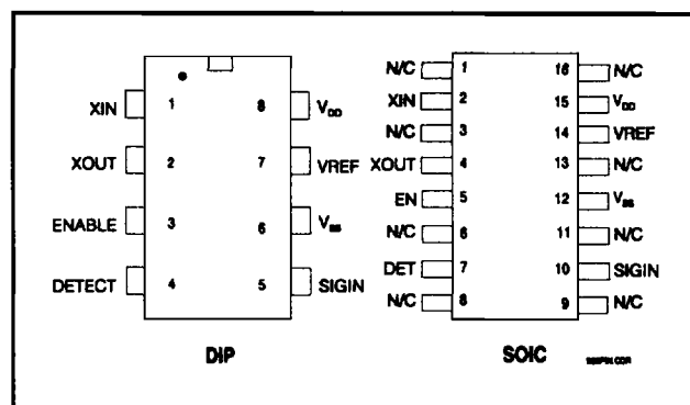
Figure 1 Pin Diagram
