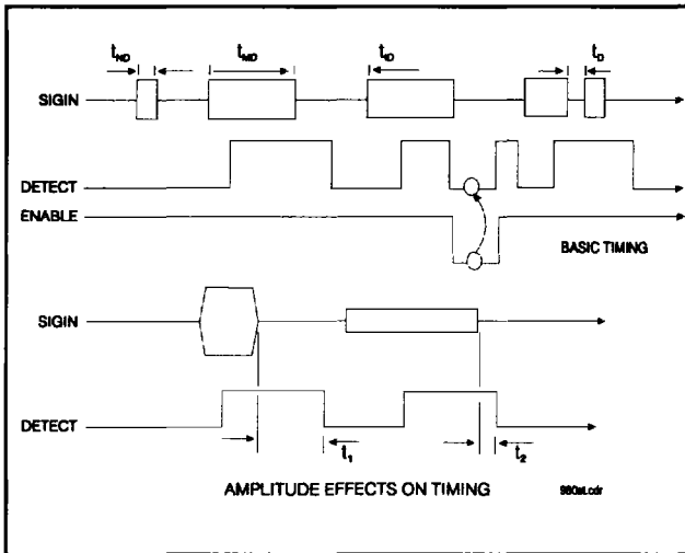
Figure 3 Signal Timing (See Table 2)
