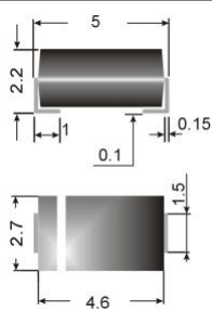
Surface mount diode
