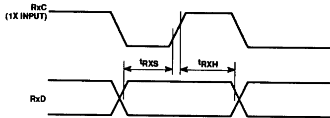
Figure 10. Receive Timing
