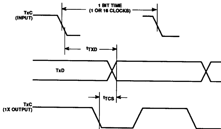
Figure 9. Transmit Timing
