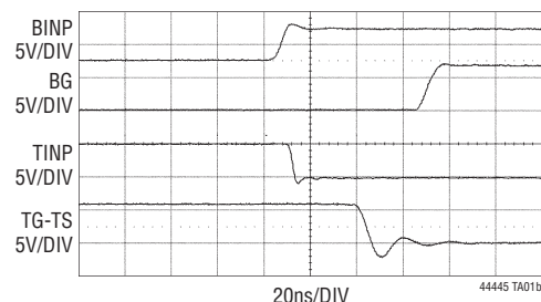
LTC4444-5 Driving a 1000pF Capacitive Load
