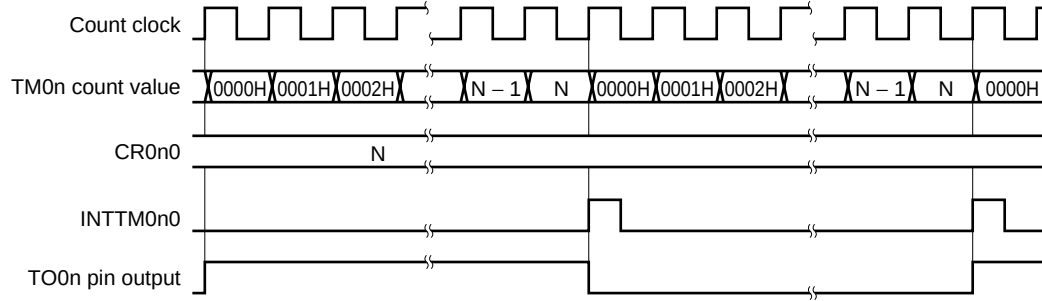
Figure 8-22. Timing of Square-Wave Output Operation
