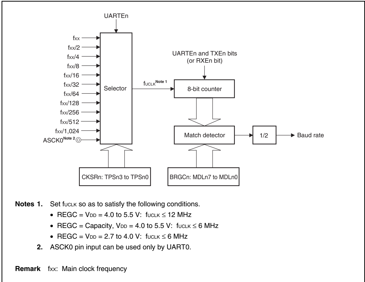
Figure 15-12. Configuration of Baud Rate Generator n (BRGn)
