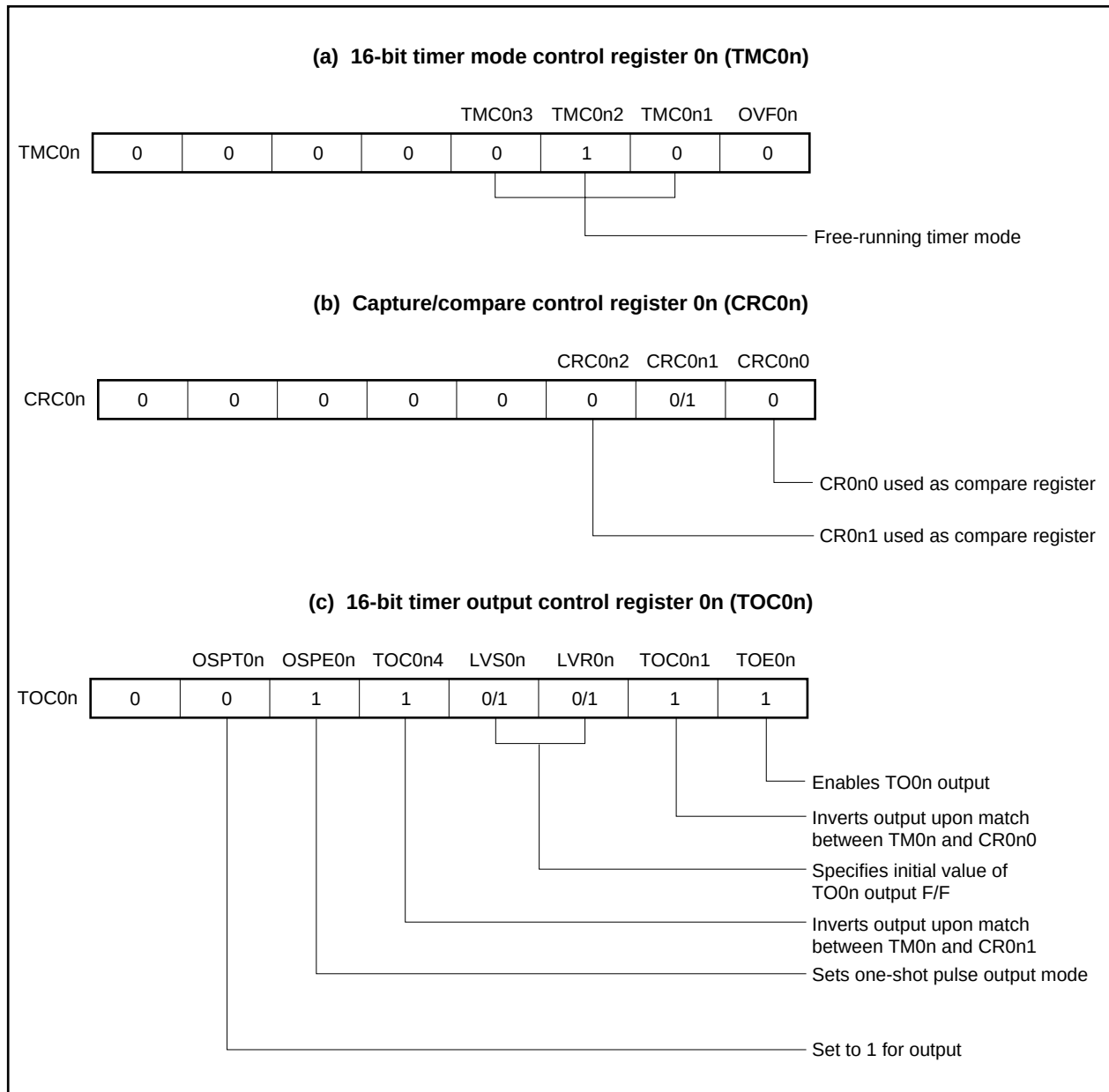
Figure 8-23. Control Register Settings for One-Shot Pulse Output (1/2)
