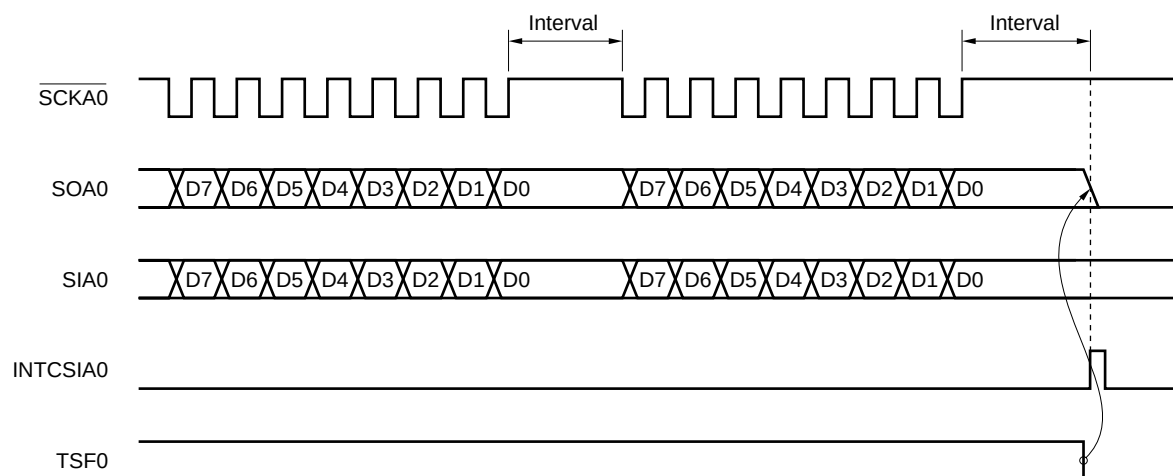
Figure 17-5. Automatic Transmission/Reception Mode Operation Timings
