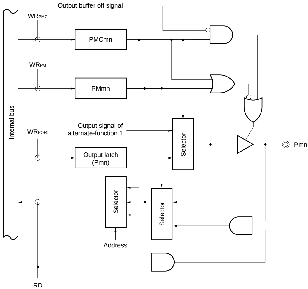
Figure 4-5. Block Diagram of Type C-3
