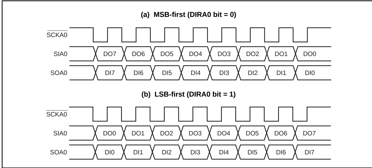
Figure 17-14. Format of CSIA0 Transmit/Receive Data
