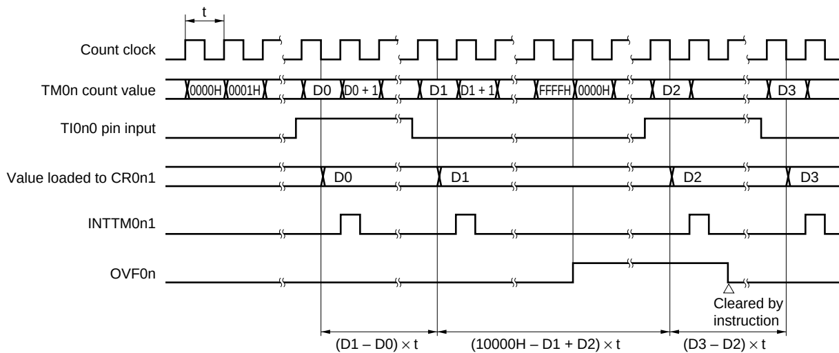
Figure 8-11. Timing of Pulse Width Measurement with Free-Running Timer Operation and One Capture Register (with Both Edges Specified)
