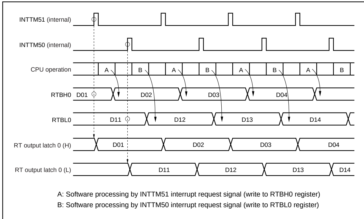
Figure 13-2. Operation Timing Example (When EXTR0 Bit = 0, BYTE0 Bit = 0)
