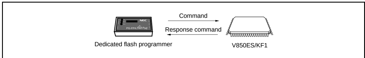
Figure 25-9. Communication Commands
