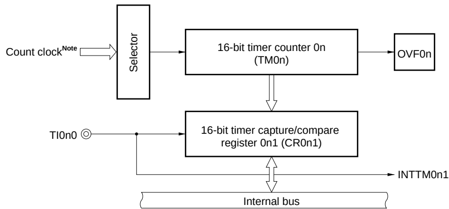
Figure 8-10. Configuration for Pulse Width Measurement with Free-Running Timer Operation
