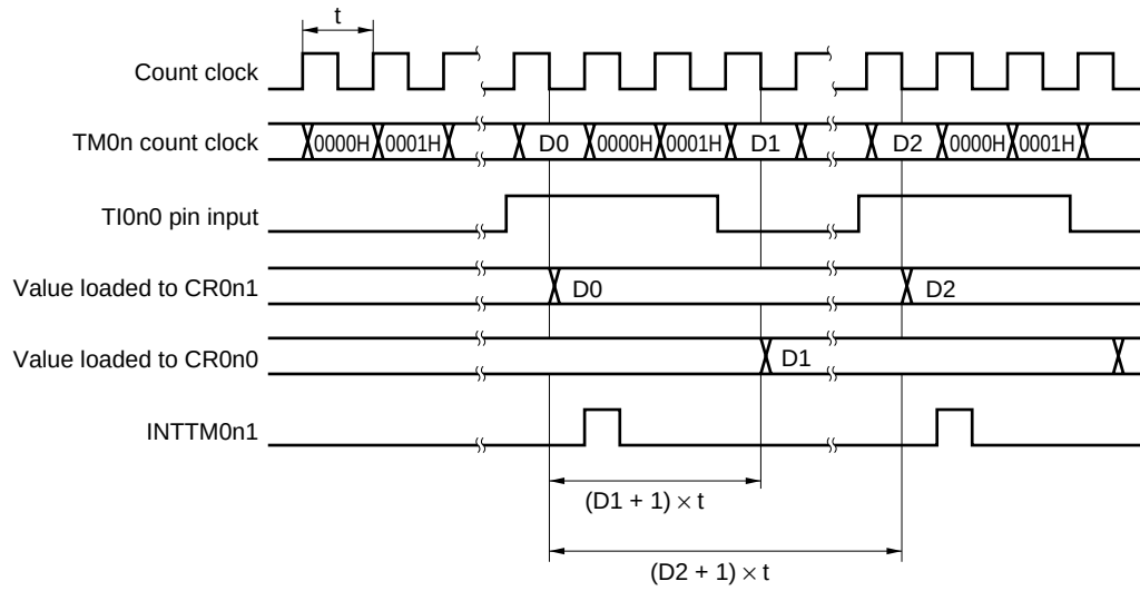
Figure 8-17. Timing of Pulse Width Measurement by Restarting (with Rising Edge Specified)
