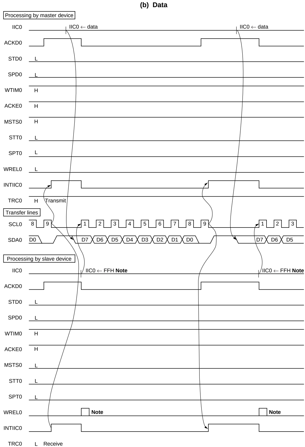
Figure 18-20. Example of Master to Slave Communication (When 9-Clock Wait Is Selected for Both Master and Slave) (2/3)
