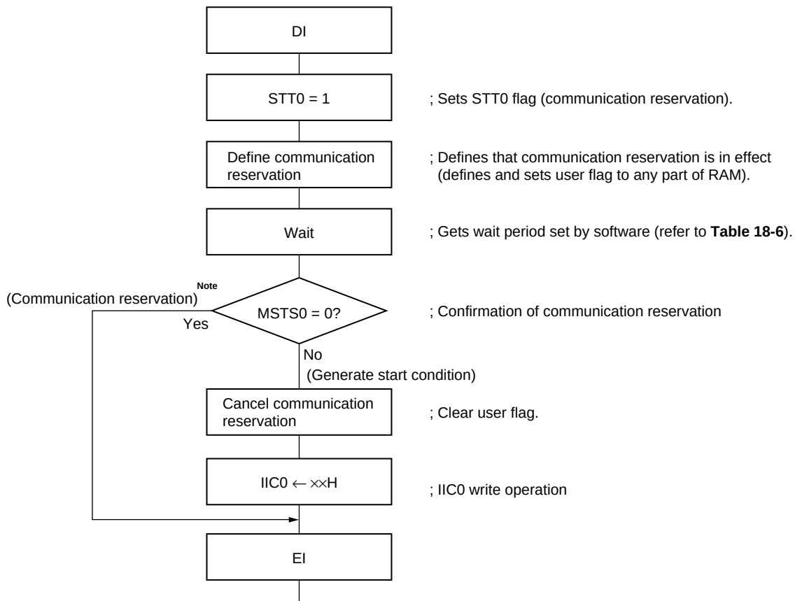
Figure 18-14. Communication Reservation Flowchart
