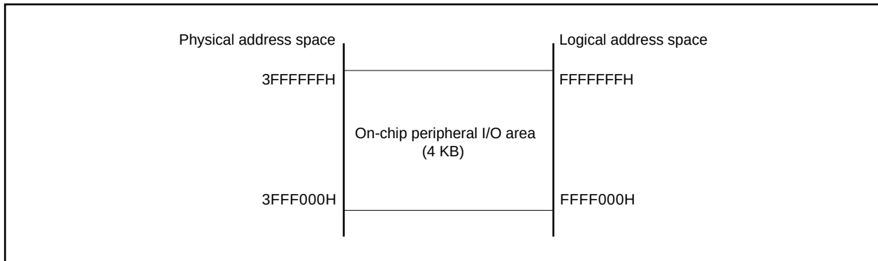
Figure 3-11. On-Chip Peripheral I/O Area
