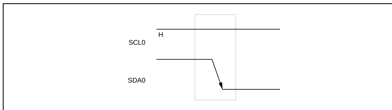
Figure 18-5. Start Conditions
