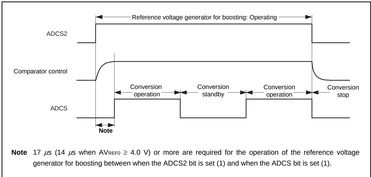
Figure 14-2. Operation Sequence
