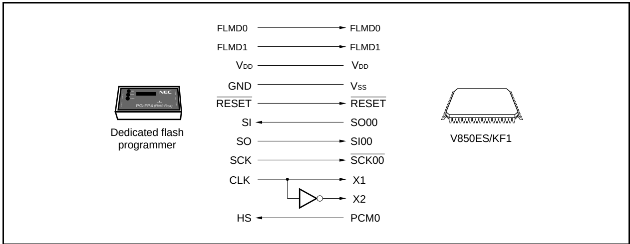
Figure 25-5. Communication with Dedicated Flash Programmer (CSI00 + HS)
