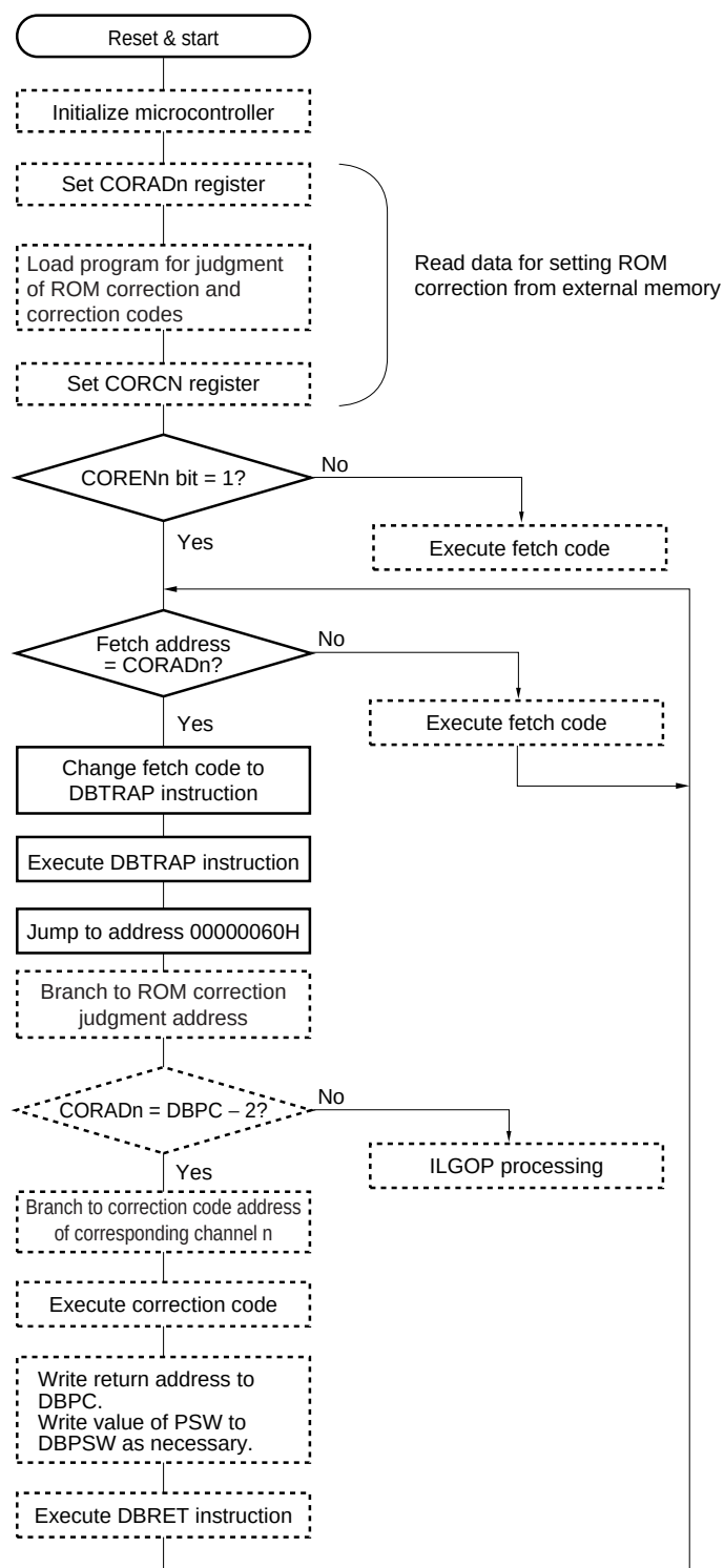
Figure 24-2. ROM Correction Operation and Program Flow
