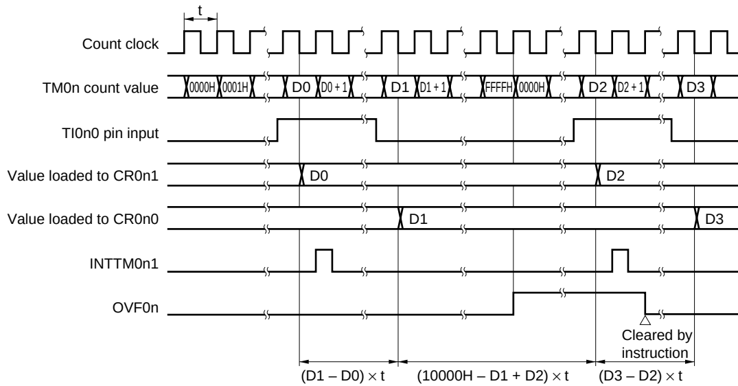
Figure 8-15. Timing of Pulse Width Measurement with Free-Running Timer Operation and Two Capture Registers (with Rising Edge Specified)
