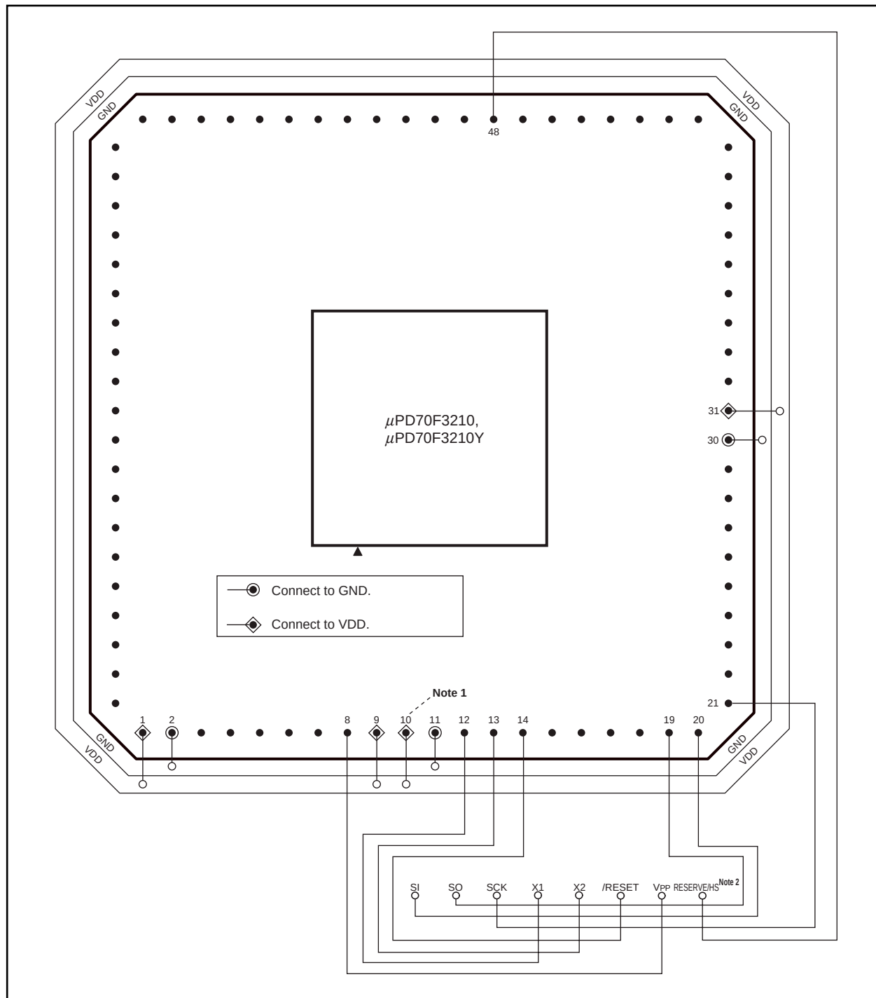
Figure 26-1. Wiring Example of V850ES/KF1 Flash Writing Adapter (FA-80GC-8BT, FA-80GK-9EU) (1/2)
