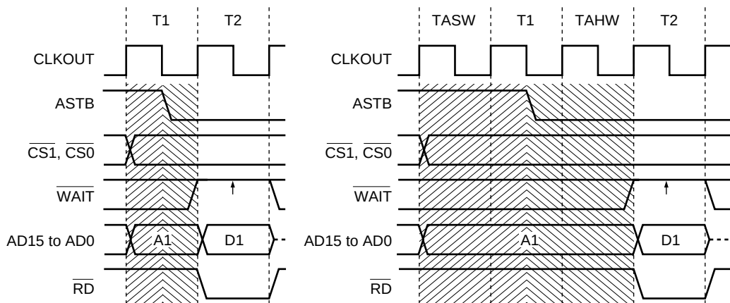
Figure 5-9. Address Wait Timing (Bus Read, Bus Size: 16 Bits, 16-Bit Access)
