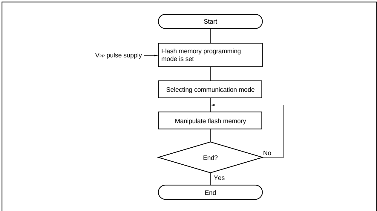
Figure 26-10. Flash Memory Manipulation Procedure
