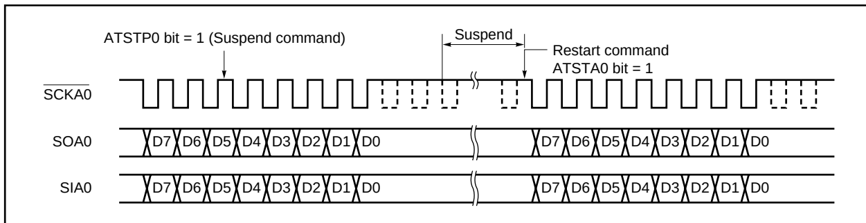
Figure 17-15. Automatic Transmission/Reception Suspension and Restart
