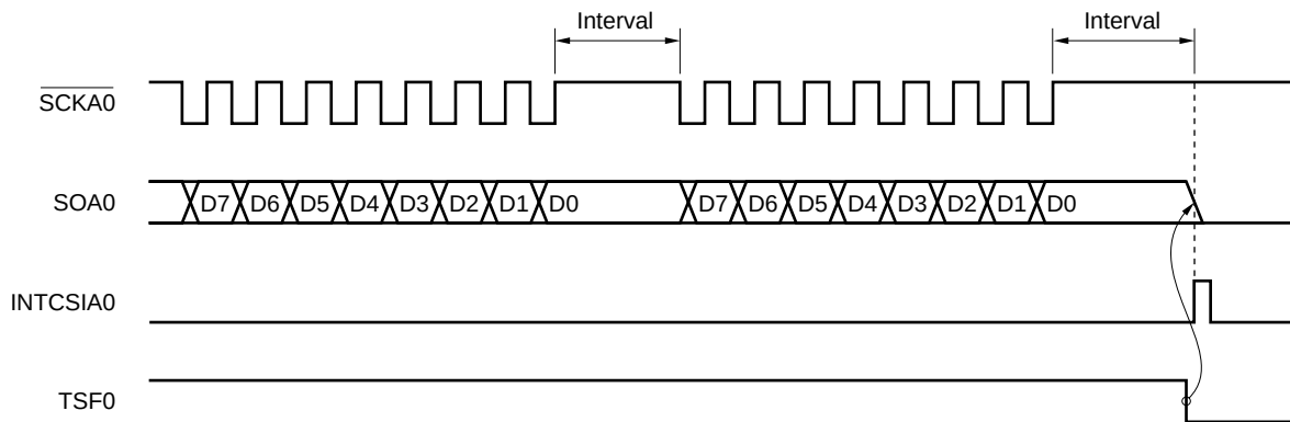
Figure 17-8. Automatic Transmission Mode Operation Timing
