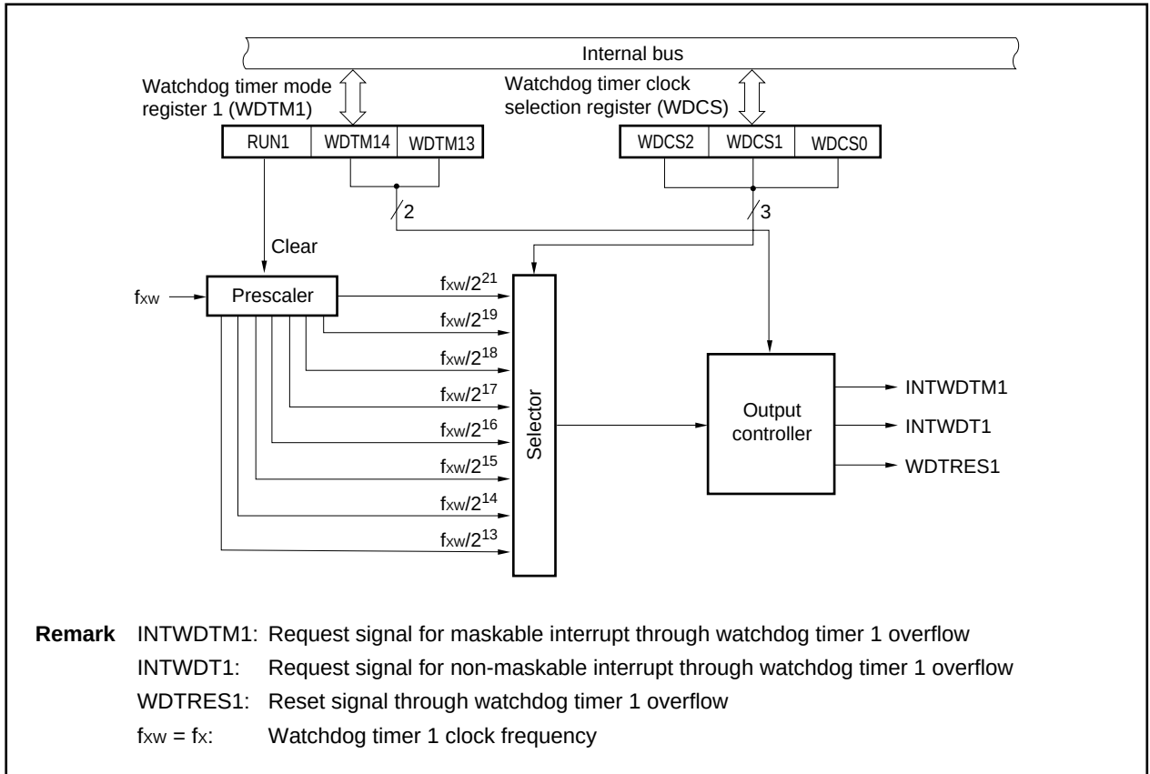
Figure 12-1. Block Diagram of Watchdog Timer 1
