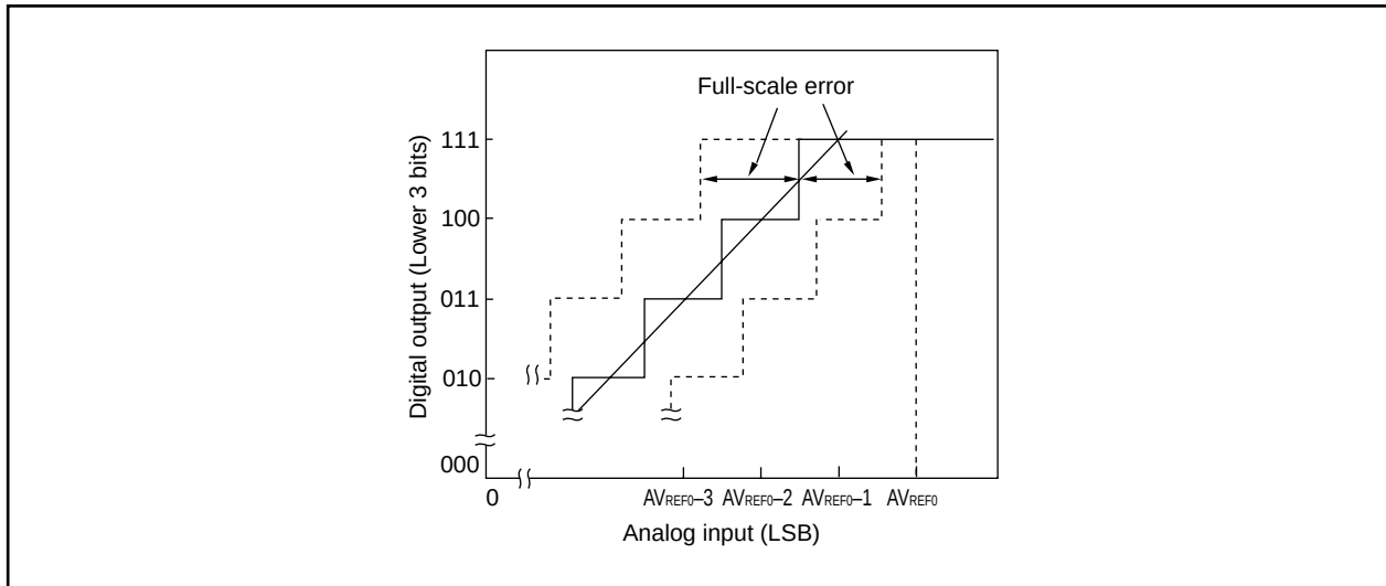
Figure 14-13. Full-Scale Error
