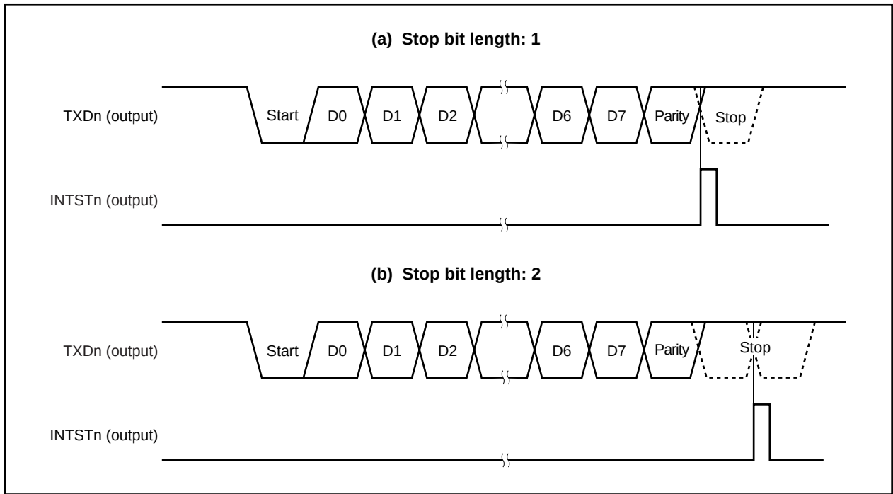
Figure 15-3. UARTn Transmission Completion Interrupt Timing
