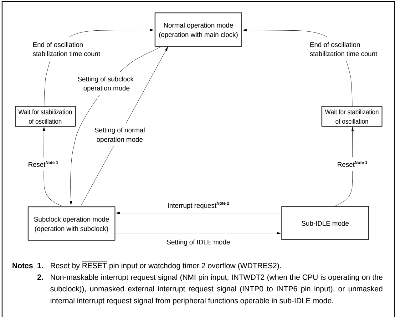
Figure 21-1. Status Transition (2/2)
