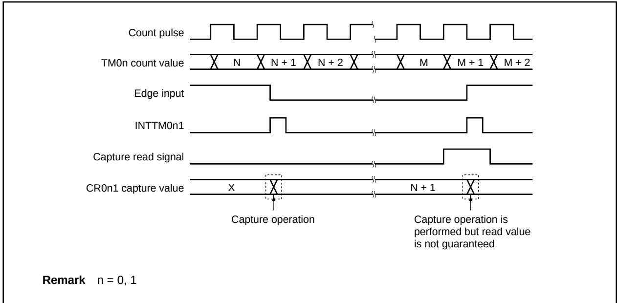
Figure 8-26. Data Hold Timing of Capture Register
