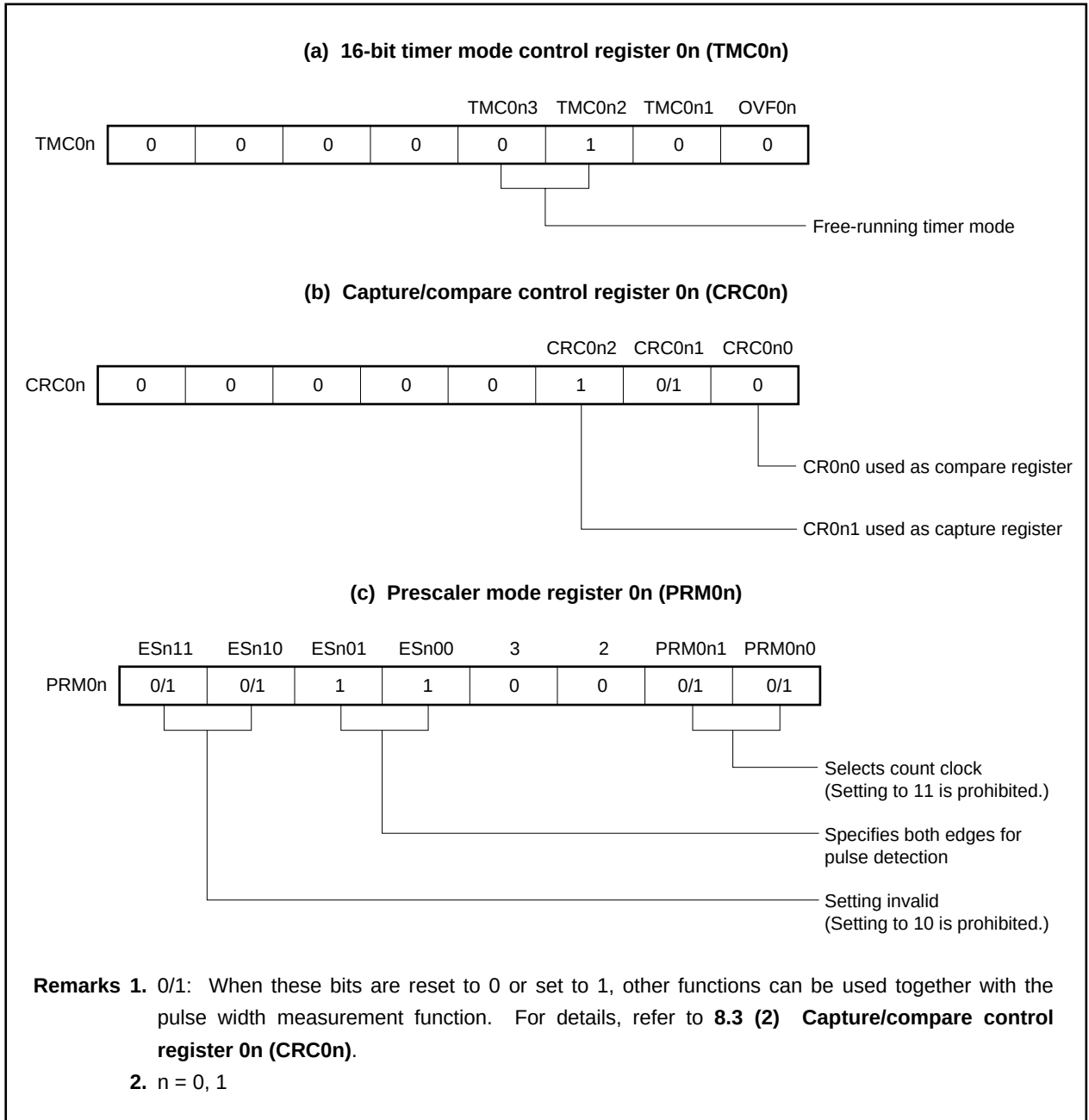
Figure 8-9. Control Register Settings for Pulse Width Measurement with Free-Running Timer Operation and One Capture Register (When TI0n0 Pin and CR0n1 Registers Are Used)
