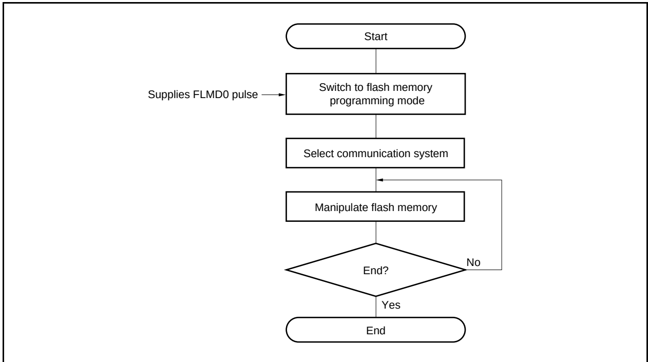
Figure 25-7. Procedure for Manipulating Flash Memory
