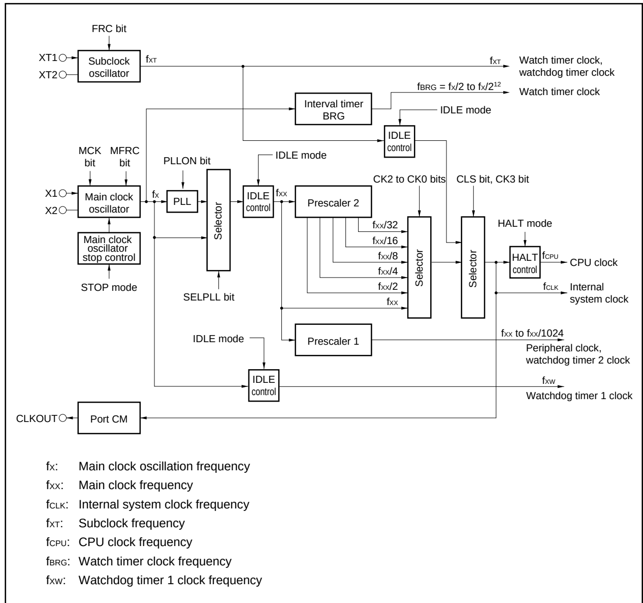
Figure 6-1. Clock Generator
