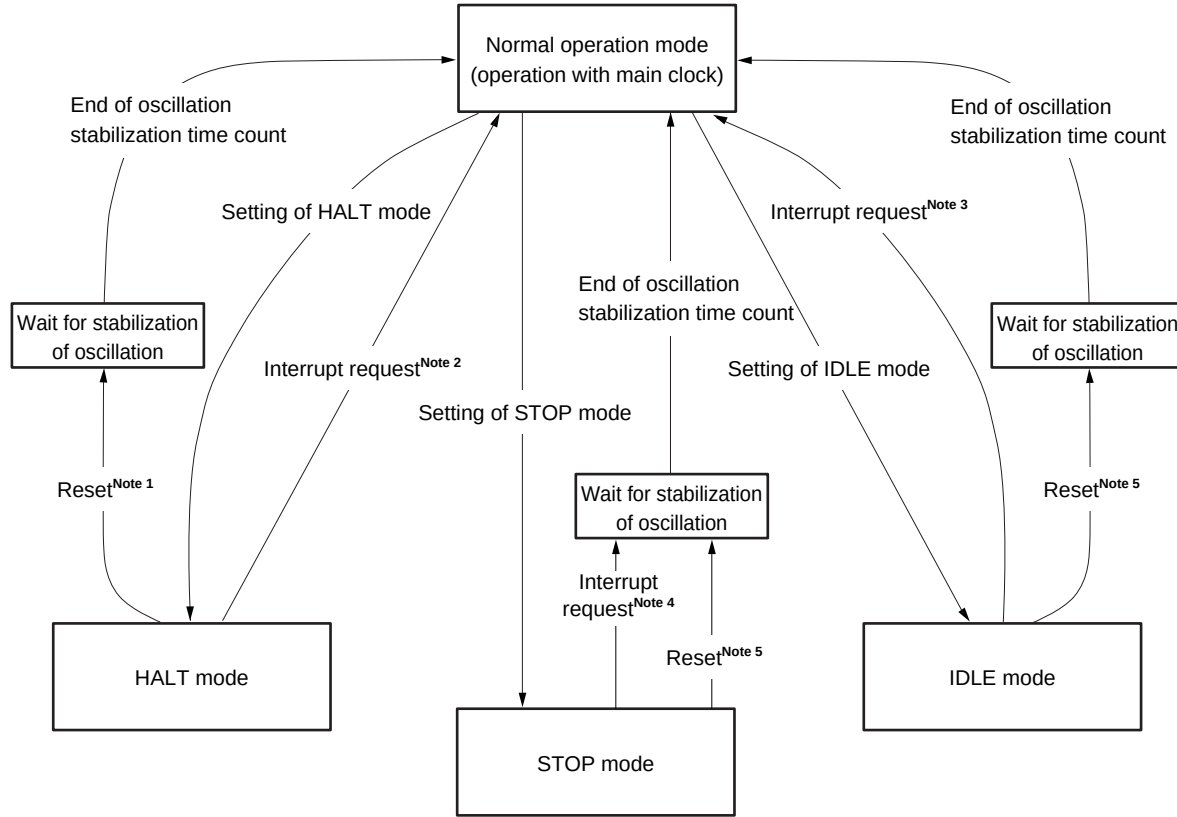
Figure 21-1. Status Transition (1/2)
