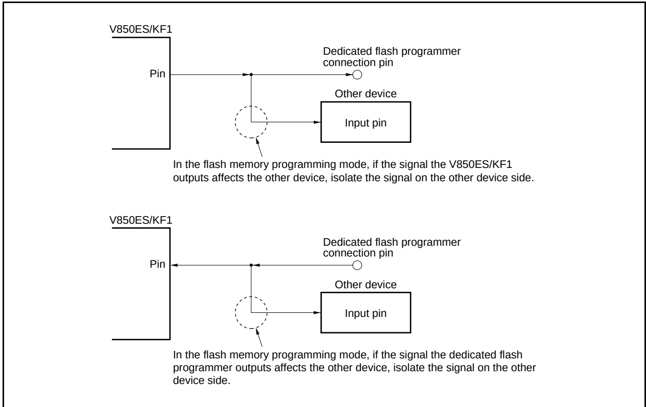
Figure 25-13. Malfunction of Other Device
