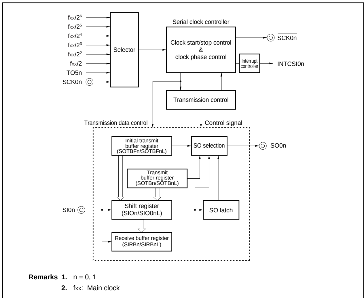
Figure 16-1. Block Diagram of Clocked Serial Interface
