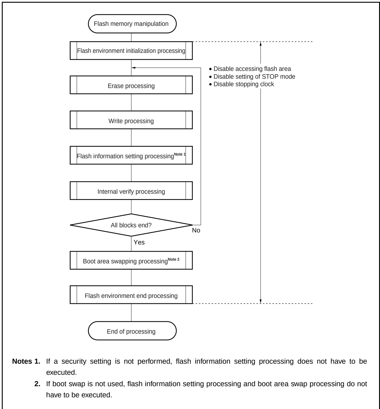
Figure 25-17. Standard Self Programming Flow
