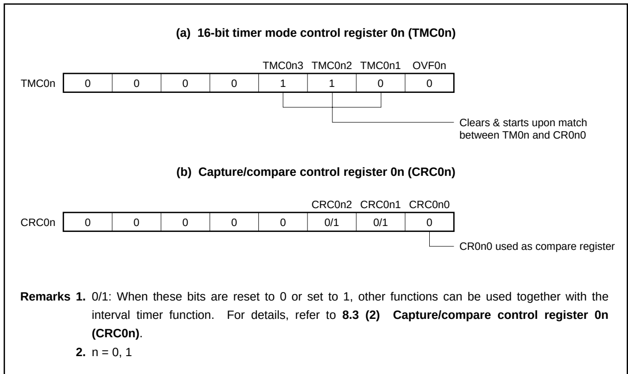
Figure 8-3. Configuration of Interval Timer
