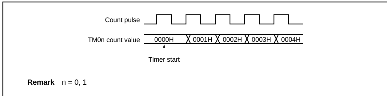
Figure 8-25. Count Start Timing of TM0n Register
