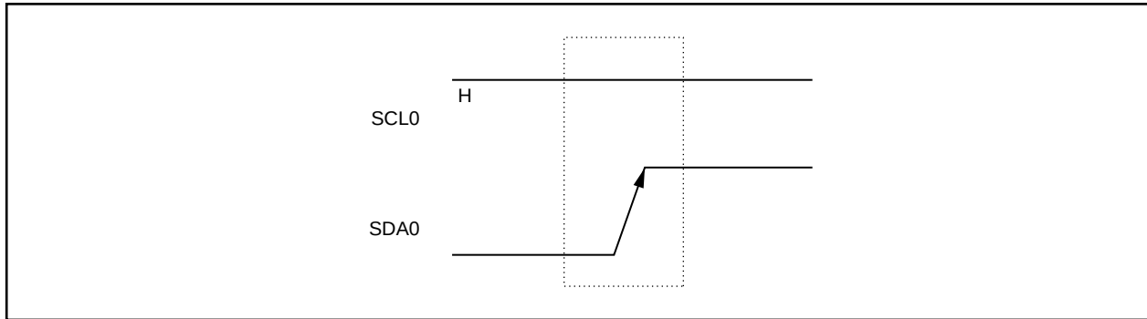
Figure 18-9. Stop Condition
