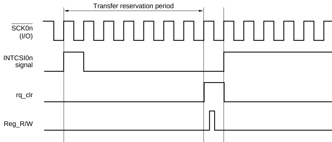
Figure 16-7. Transfer Request Clear and Register Access Conflict
