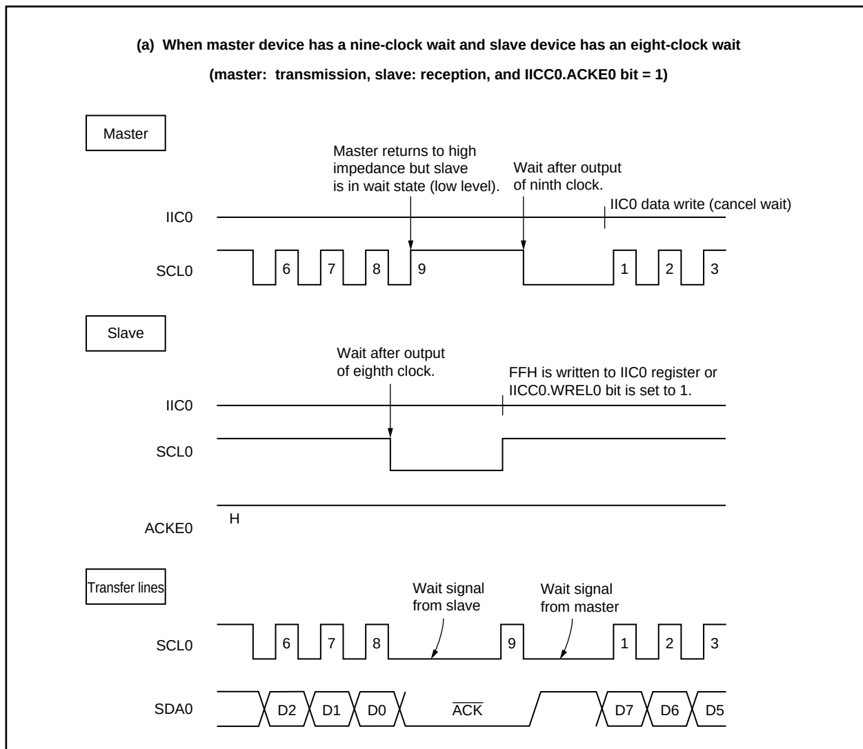
Figure 18-10. Wait Signal (1/2)
