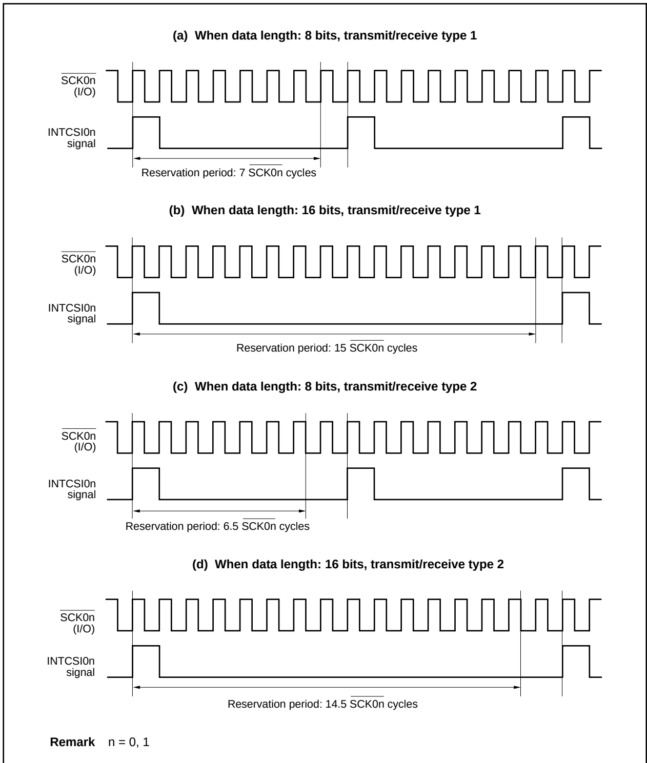
Figure 16-6. Timing Chart of Next Transfer Reservation Period
