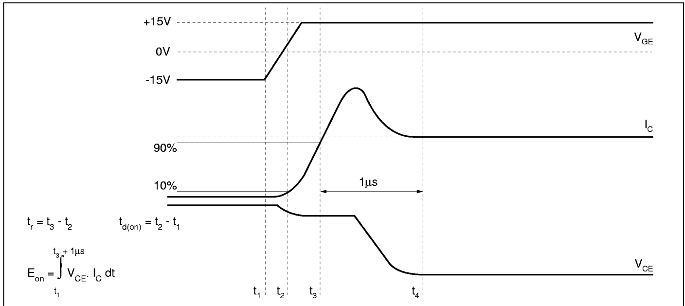
Fig.4 Turn-on characteristics
