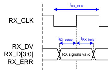
Figure 5: MII timing RX signals
