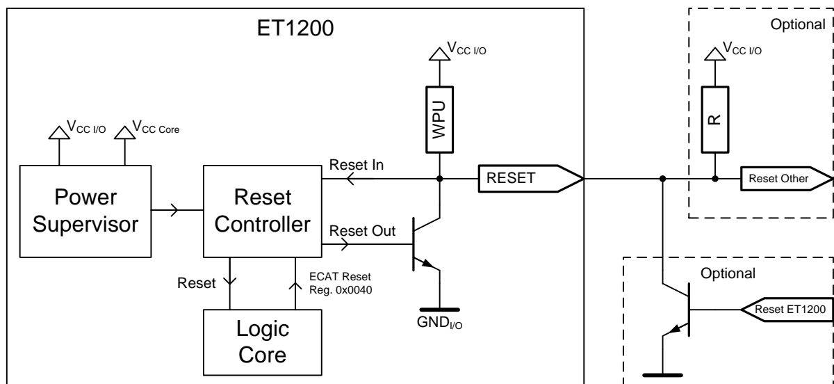
Figure 31: Reset Logic
