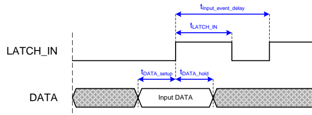
Figure 11: Digital Input: Input data sampled with LATCH_IN
