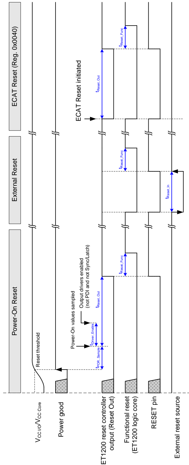
Figure 32: Reset Timing
