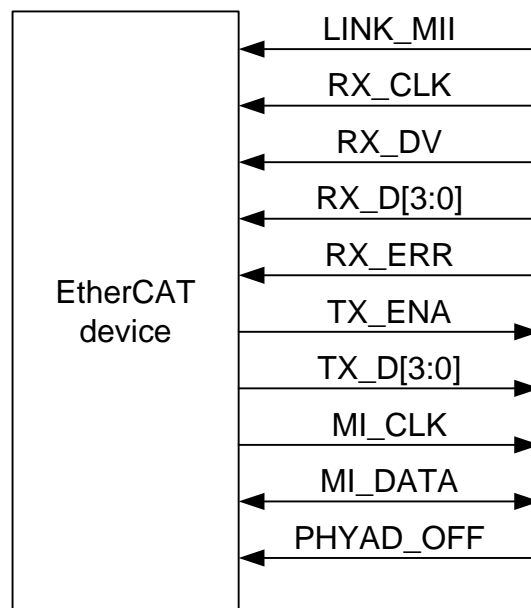
Figure 3: MII Interface signals
