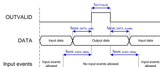
Figure 13: Bidirectional Mode timing
