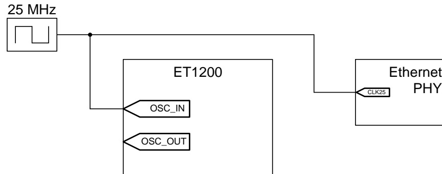
Figure 25: Oscillator clock source for ET1200 and Ethernet PHYs
