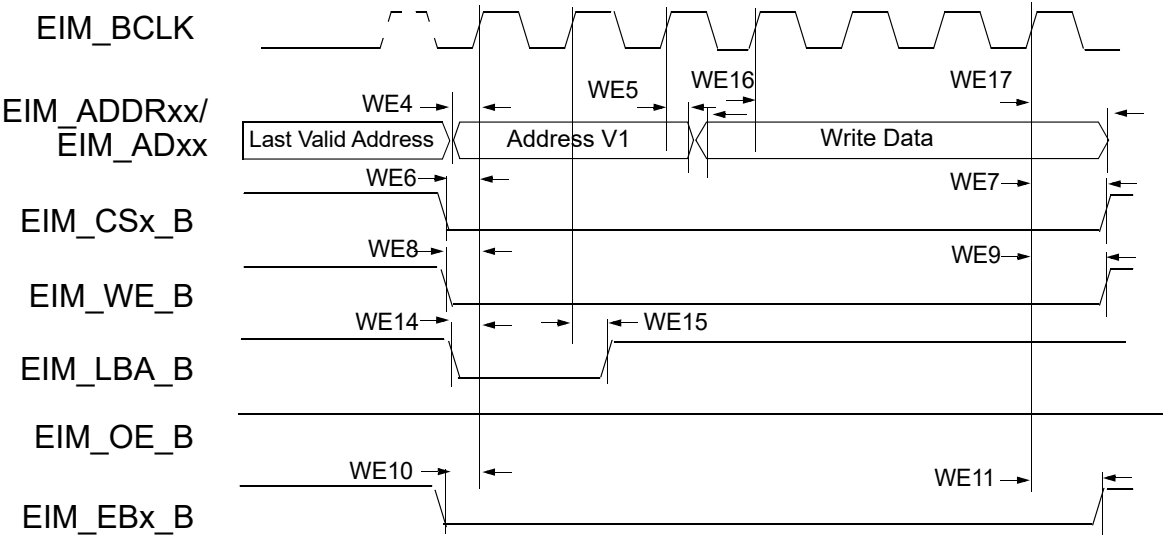
Figure 15. Muxed Address/Data (A/D) Mode, Synchronous Write Access, WSC=6, ADVA=0, ADVN=1, and ADH=1
