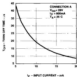
Figure 15. Typical Turn Off Time vs. Input Current.
