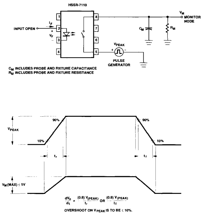
Figure 17. Output Transient Rejection Test Circuit.
