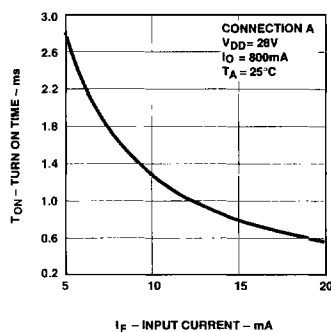
Figure 12. Typical Turn On Time vs. Input Current.
