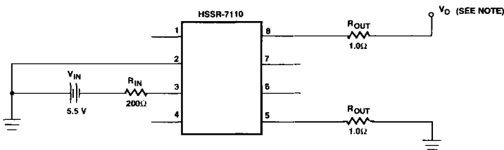
Figure 20. Burn-In Circuit.
