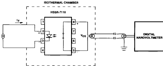
Figure 19. Voltage Offset Test Setup.
