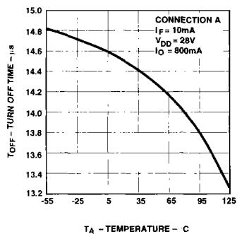
Figure 14. Typical Turn Off Time vs. Temperature.
