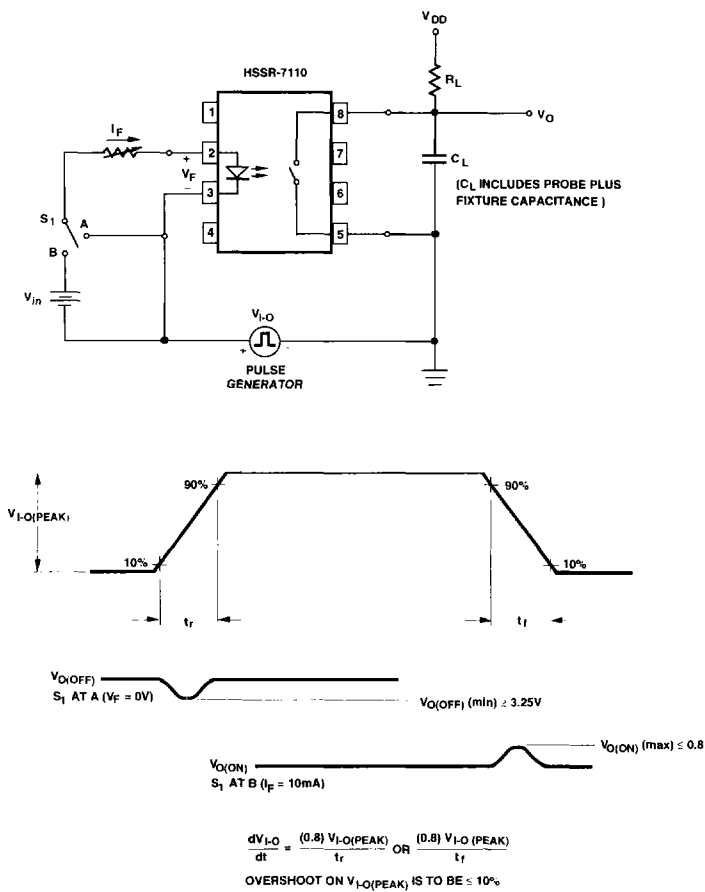
Figure 18. Input-Output Transient Rejection Test Circuit.
