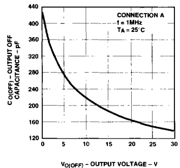
Figure 16. Typical Output Off Capacitance vs. Output Voltage.
