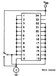
Fig. 17 - Quiescent device current test circuit.
