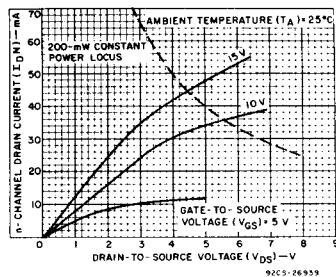
Fig.2 — Minimum output n-channel drain characteristics.
