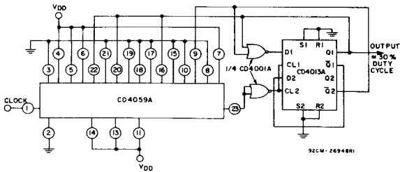
Fig. 16 - Division by 47,690 in \pm 2 mode.
