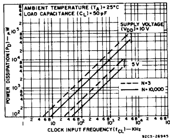
Fig. 13 - Typical power dissipation vs. clock input frequency.
