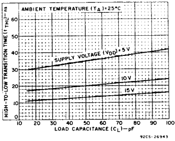
Fig. 10 - Typical high-to-low transition time vs. load capacitance.
