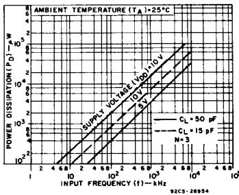
Fig. 12 - Typical power dissipation vs. input frequency.
