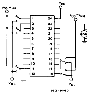
Fig. 18 - Noise immunity test circuit.
