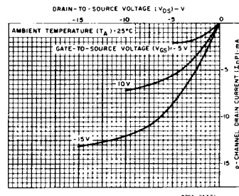
Fig.4 — Minimum output p-channel drain characteristics.
