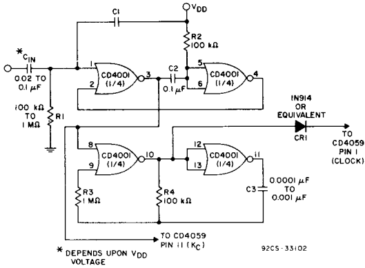
Fig.21 - CD4059A mode 5 power on master preset circuit.
