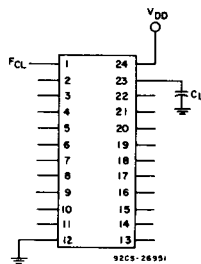
Fig. 19 - Power dissipation test circuit (all \pm modes).
