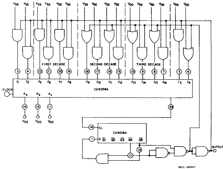
Fig. 15 - Dividing by any number from 88,003 to 103,999.
