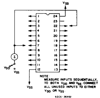
Fig. 20 - Input leakage current test circuit.
