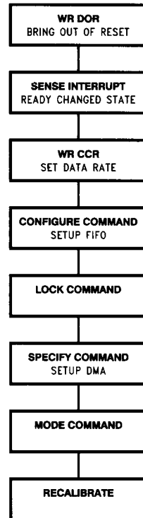
FIGURE 7-2. PC8477B Initialization
