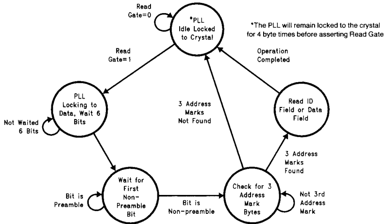
FIGURE 5-2. Read Data Algorithm—State Machine
