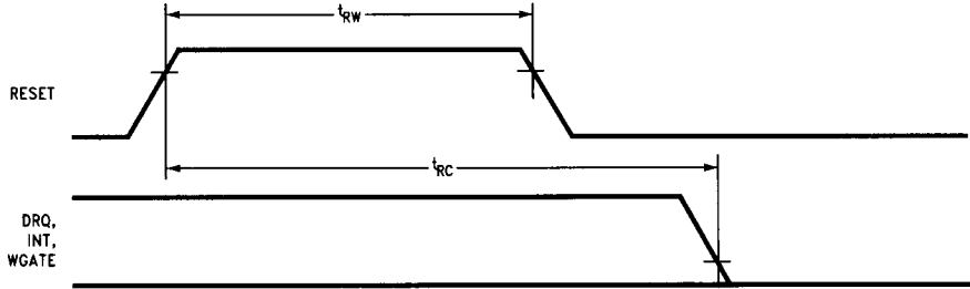
FIGURE 6-5. Reset Timing
