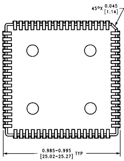
Plastic Chip Carrier (V) Order Number PC8477BV-1 NS Package Number VA68A
