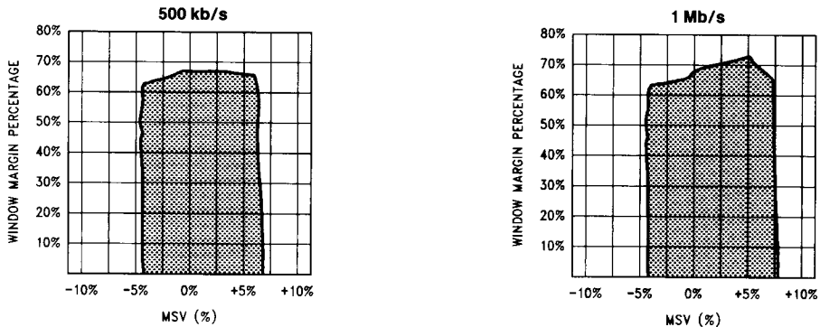
FIGURE 5-4. PC8477B Dynamic Window Margin Performance with \pm 3\% ISV at 1 kHz (Typical performance at V_{CC} = 5.0V , 25^{\circ}C )
