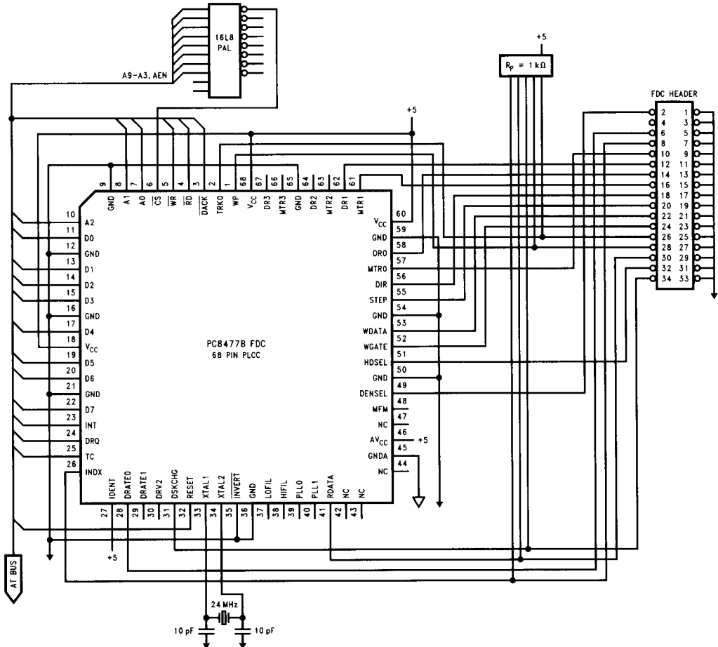
FIGURE 7-1. 8477B in PC-AT System
