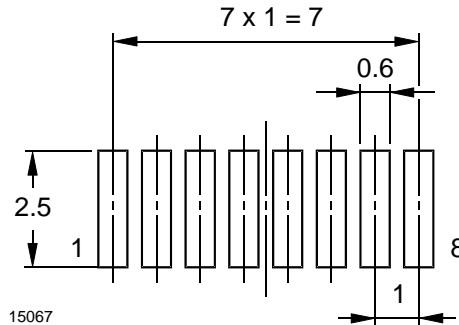
Figure 7. TFDH6131 Side View Package
