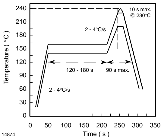
Figure 9. Recommended Solder Profile
