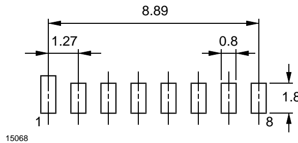
Figure 8. TFDH6541 Side View Package
