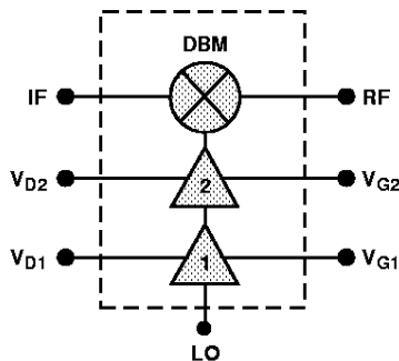
Figure 1. Simplified Block Diagram.
