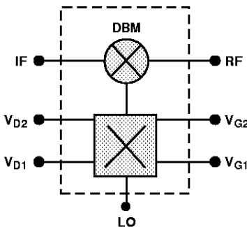
Figure 2. Harmonic Mixing Block Diagram.
