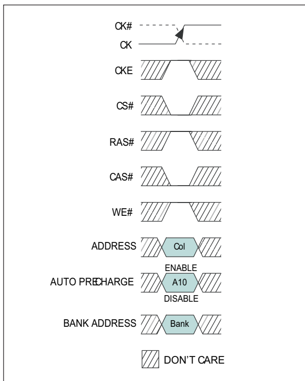
FIGURE 11 – READ COMMAND
