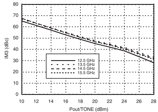
Output IM3 @ Vdd = +7V
