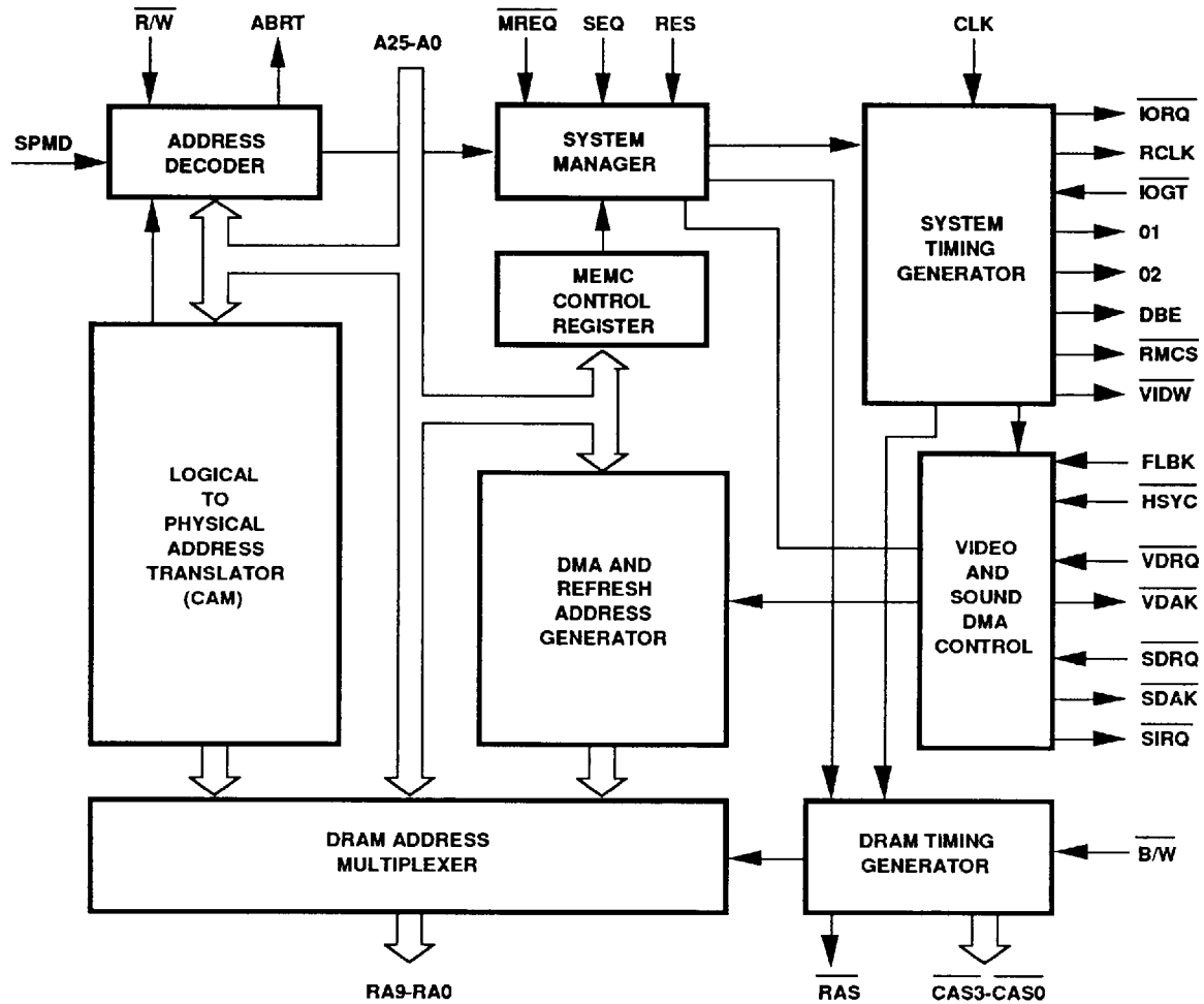
VY86C110 RISC MEMORY CONTROLLER BLOCK DIAGRAM
