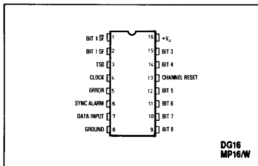
Fig.1 Pin connections
