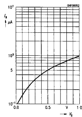
Dark current I_R = f(V_R), E = 0
