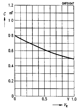
Capacitance C = f(V_R), f = 1 \text{ MHz}, E = 0
