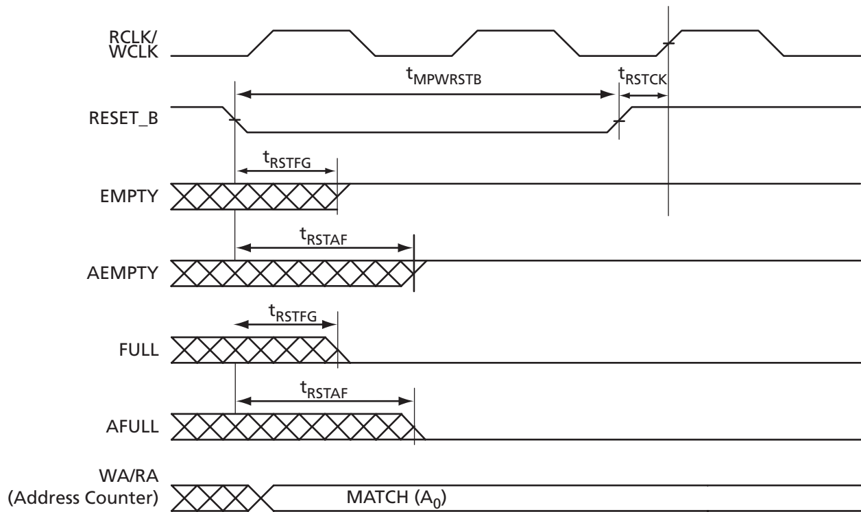
Figure 2-40 • FIFO Reset
