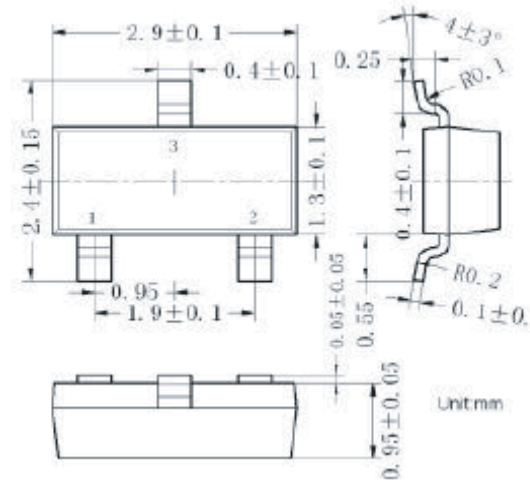
1.BASE 2.EMITTER 3.COLLECTOR
