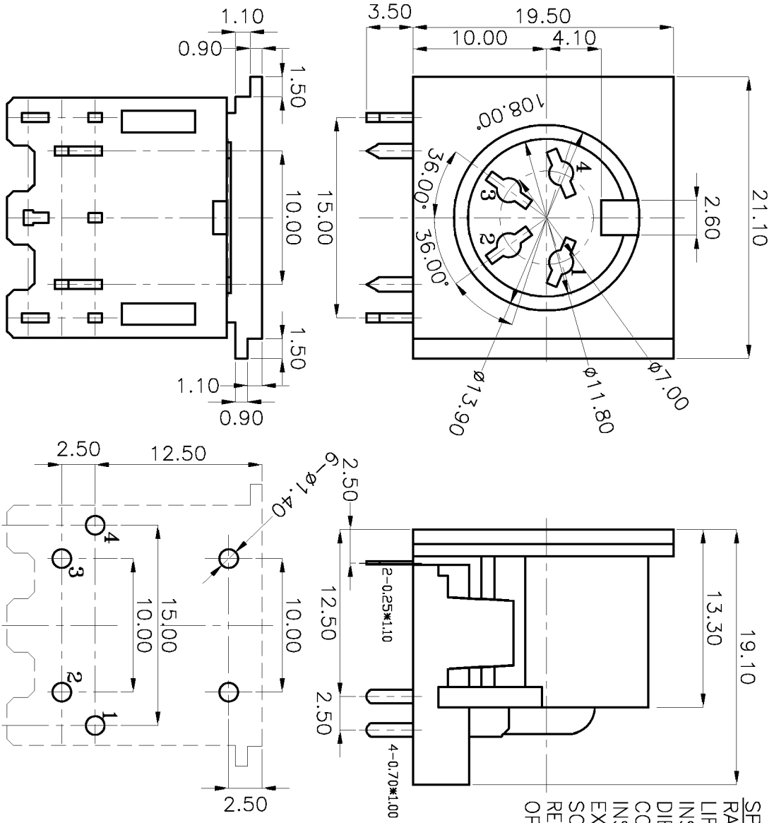
PCB LAYOUT (BOTTOM VIEW)
