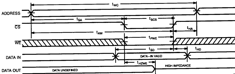
Write Cycle No. 2 ( \overline{CS} Controlled) [7,10]
