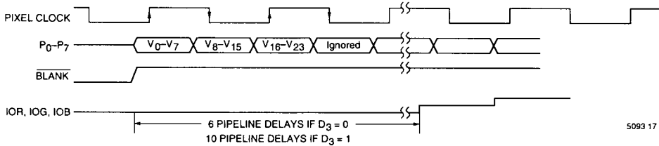
Figure 13. Repack Mode 3a Timing
