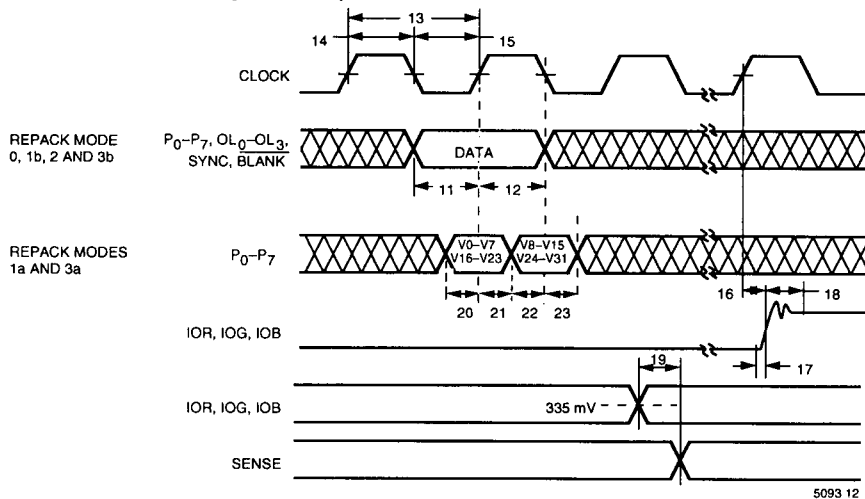
Figure 8. Video Input/Output Timing
