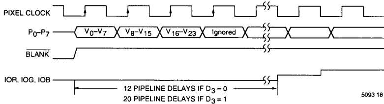
Figure 14. Repack Mode 3b Timing
