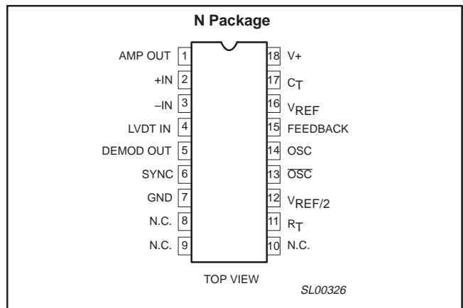
Figure 1. Pin configurations
