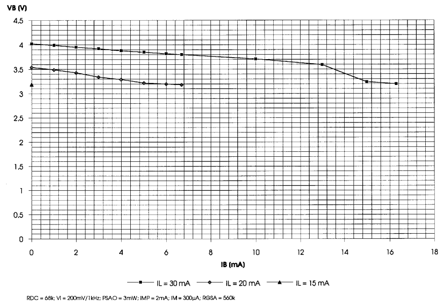
Figure 18. Typical Load Characteristic of V_B for a Minimum DC Characteristic ( R_{DC} = 68\text{ k}\Omega ) and a 3-mW Loudspeaker Output
