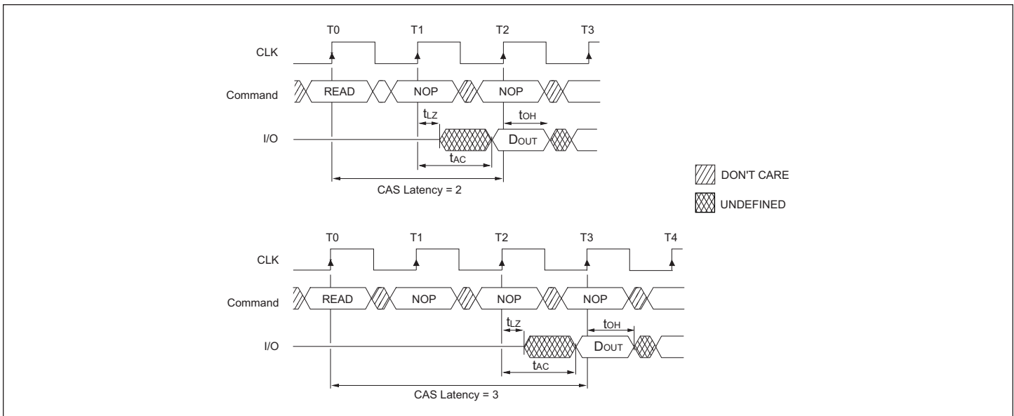
FIGURE. 4 – CAS LATENCY
