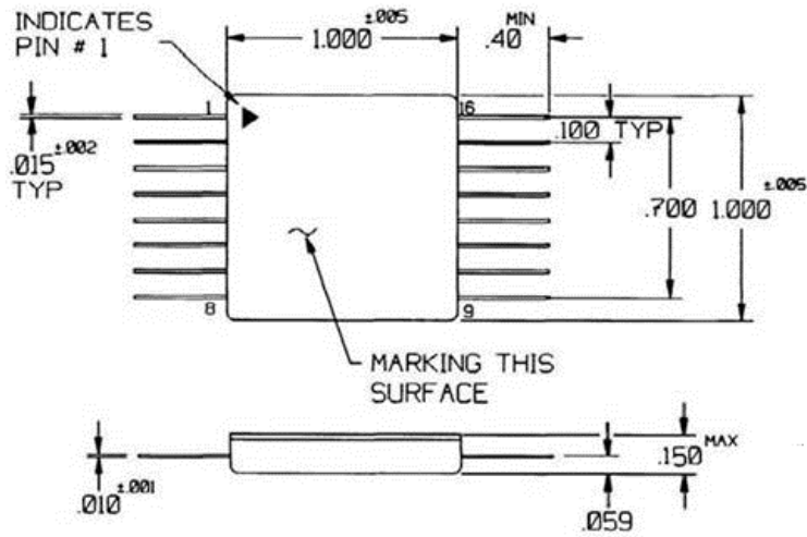
FIGURE 3 Model 5219 Package Outline
