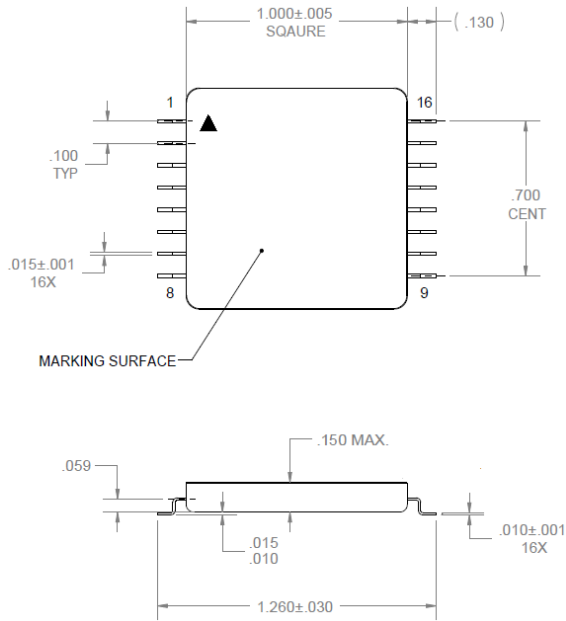
FIGURE 4 Model 5221 Package Outline
