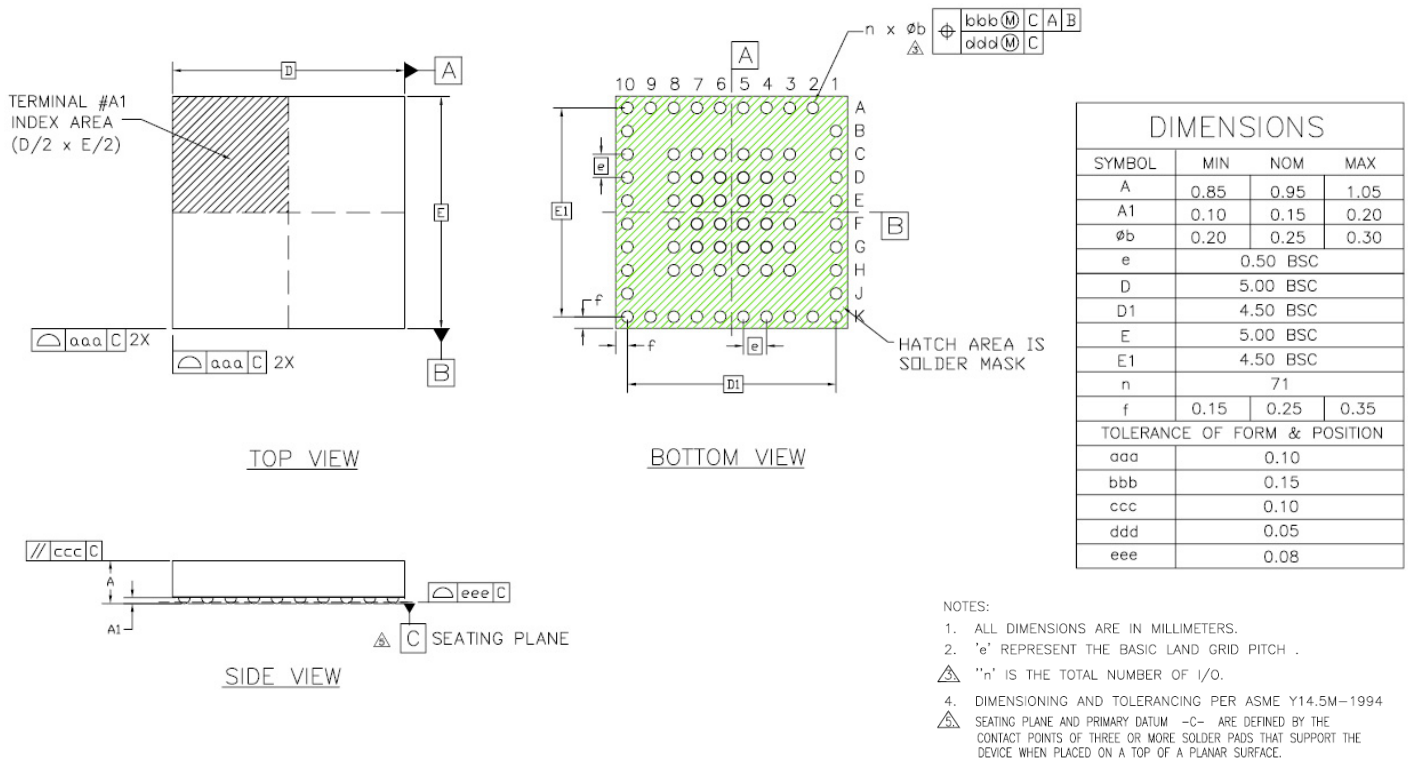
Figure 29. NAG/HLA Package Outline
