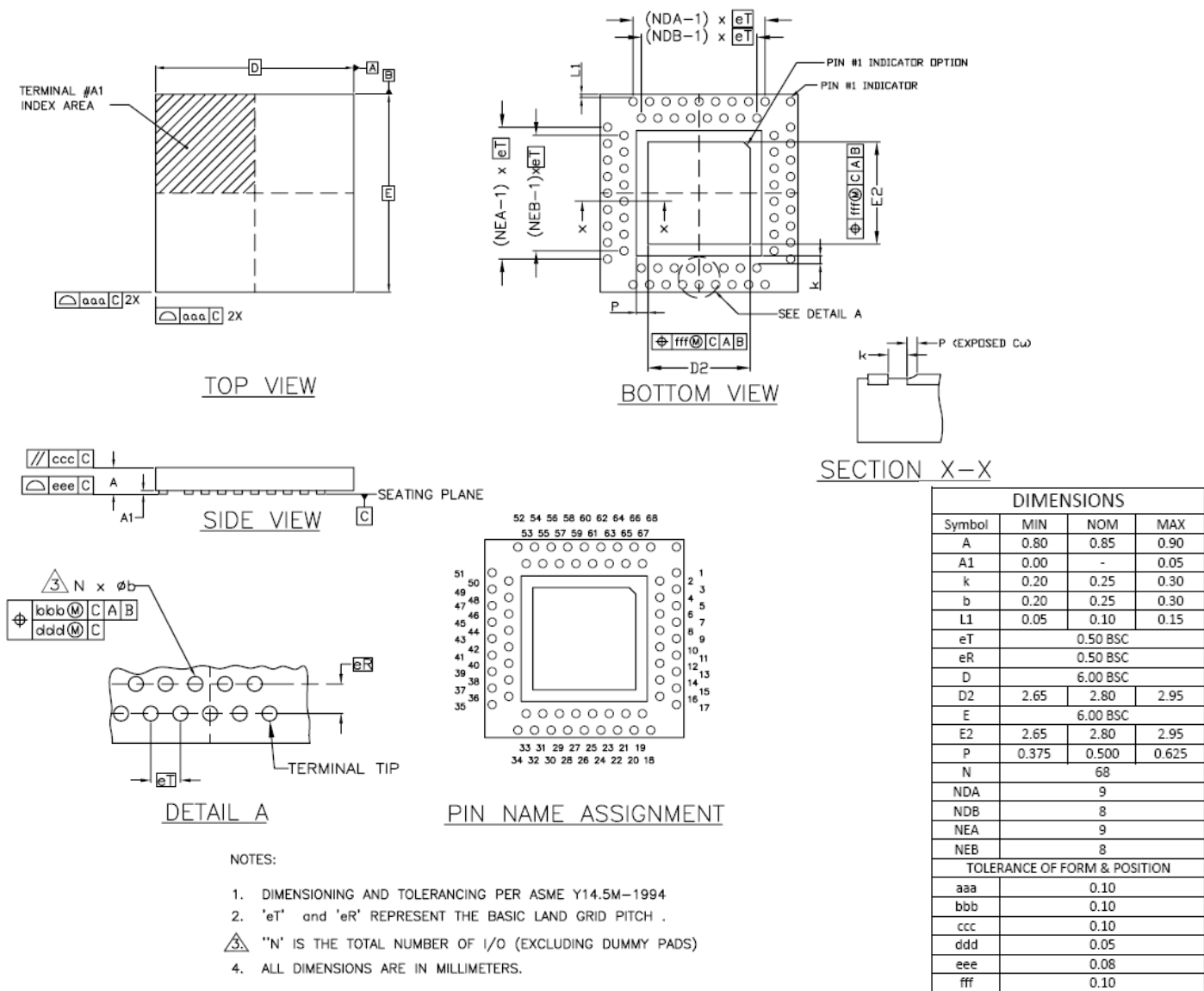
Figure 28. Package Outline
