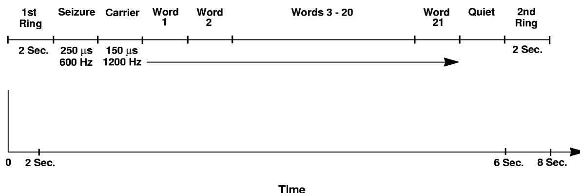
Figure 10-4. Caller ID Signal Timing
