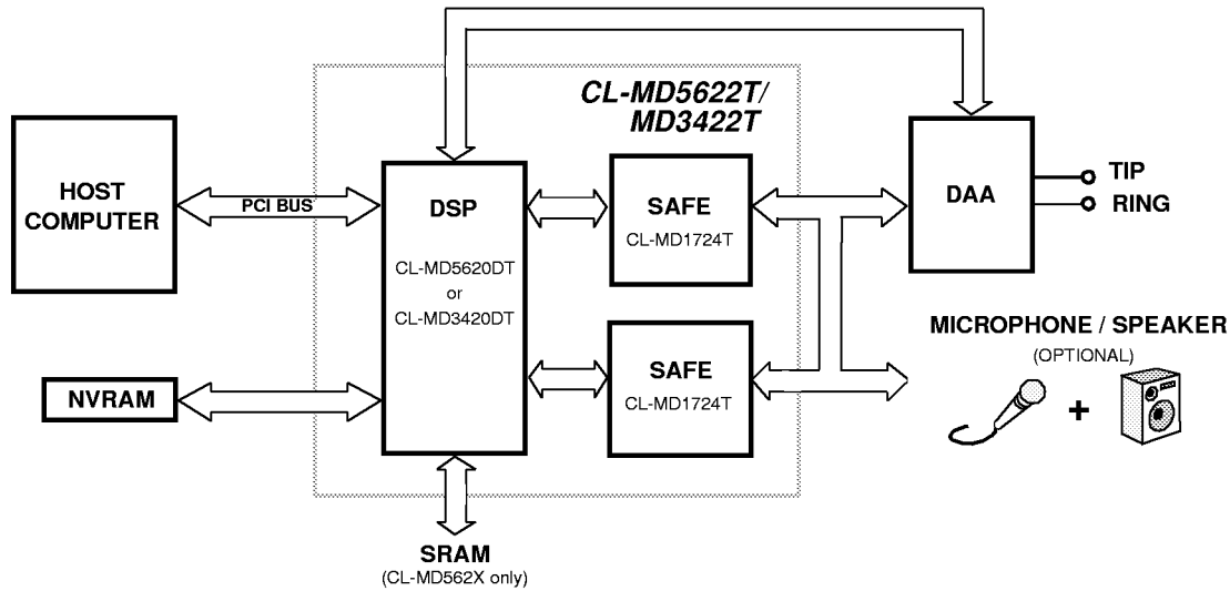
Figure 1-3. CL-MD5622T/MD3422T Functional Block Diagram
