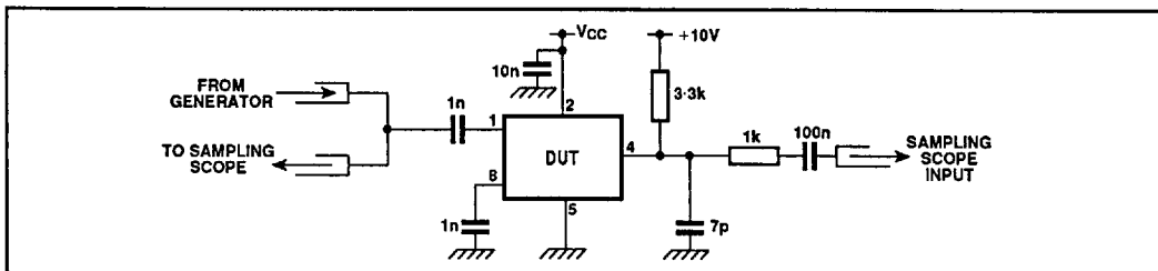
Fig. 5 Test circuit
