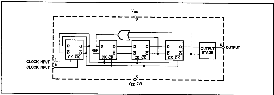
Fig. 2 Functional diagram
