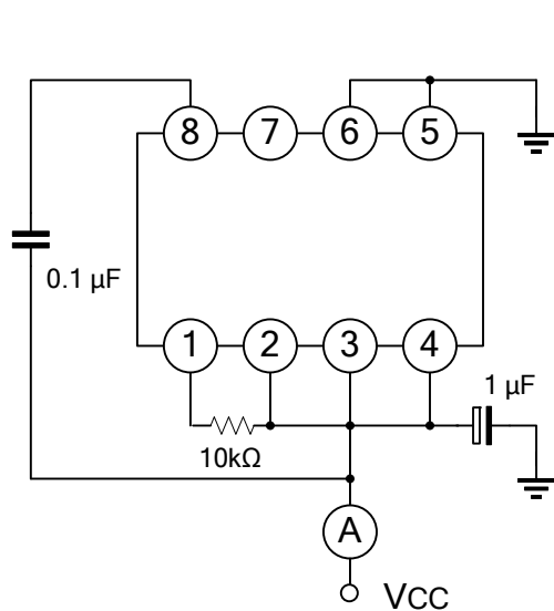
Fig.1 ( I_{CC}, \frac{\Delta V_{REF}}{V_{REF}} / \Delta V_{CC} )
