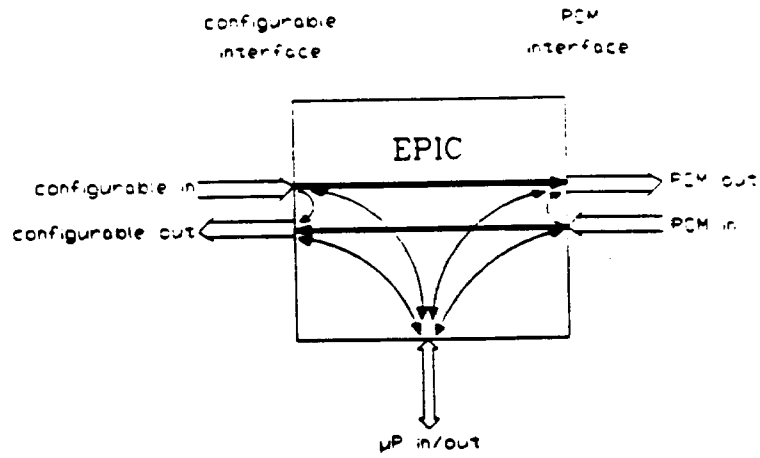
Figure 2.4: Transmission and Access Possibilities of the EPIC
