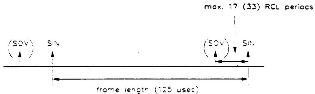
Figure 2.6: Synchron Transfer Flow Diagram
