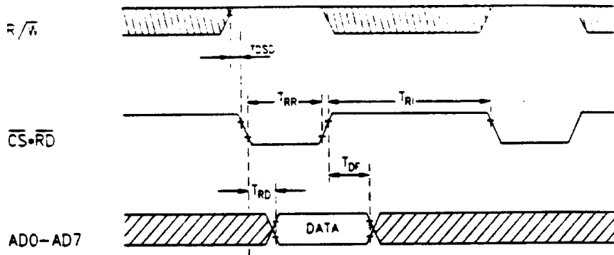
Fig. 5.6: \mu P Read Cycle
