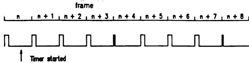
Fig. 4.4: FSC output signal in FSC mode 7
