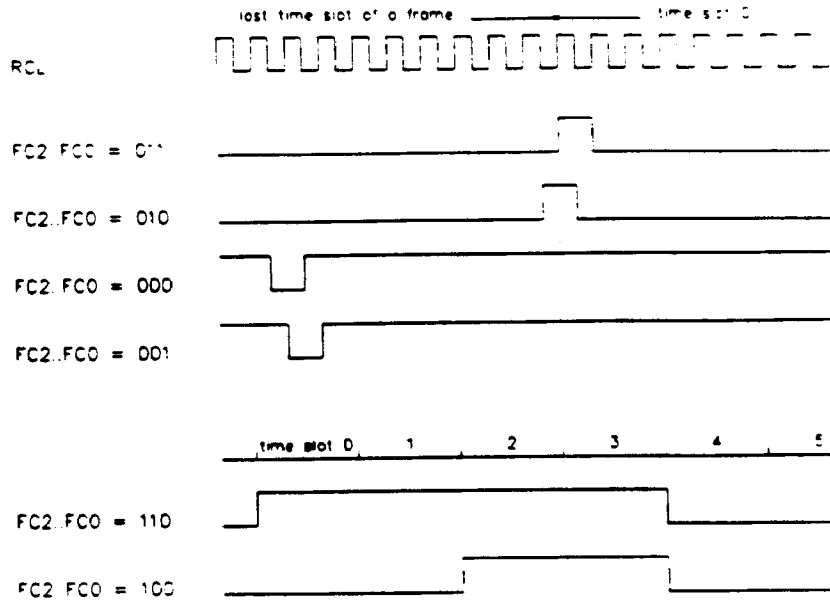
Fig. 4.3: FSC Framing Signal Generation
