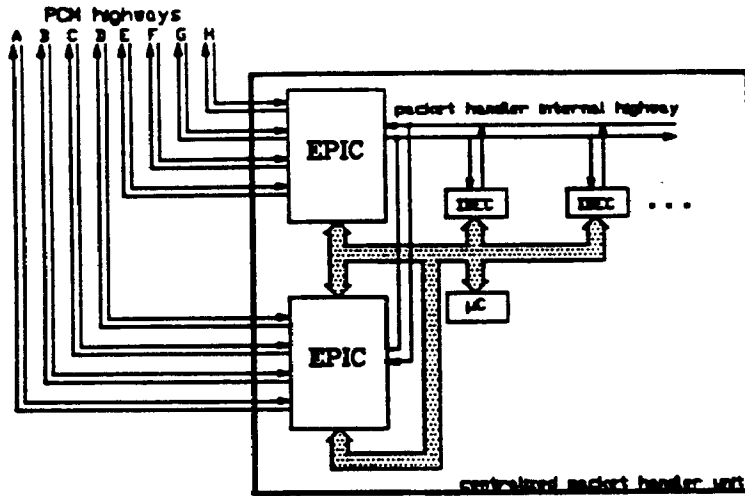
Fig. 1.11: Centralized Packet Handler with One Internal Highway Connected to 8 PCM Highways
