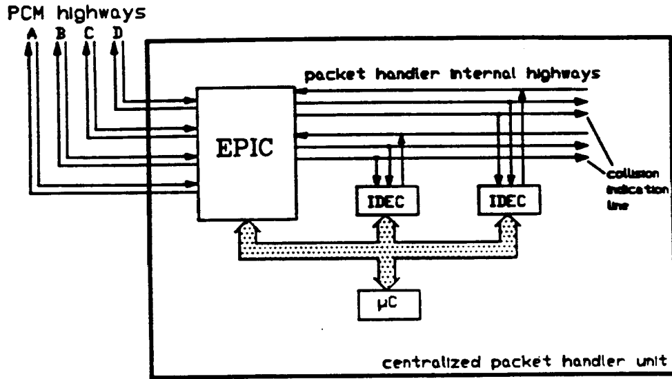
Fig. 1.13: Centralized Packet Handler with Internal Collision line
