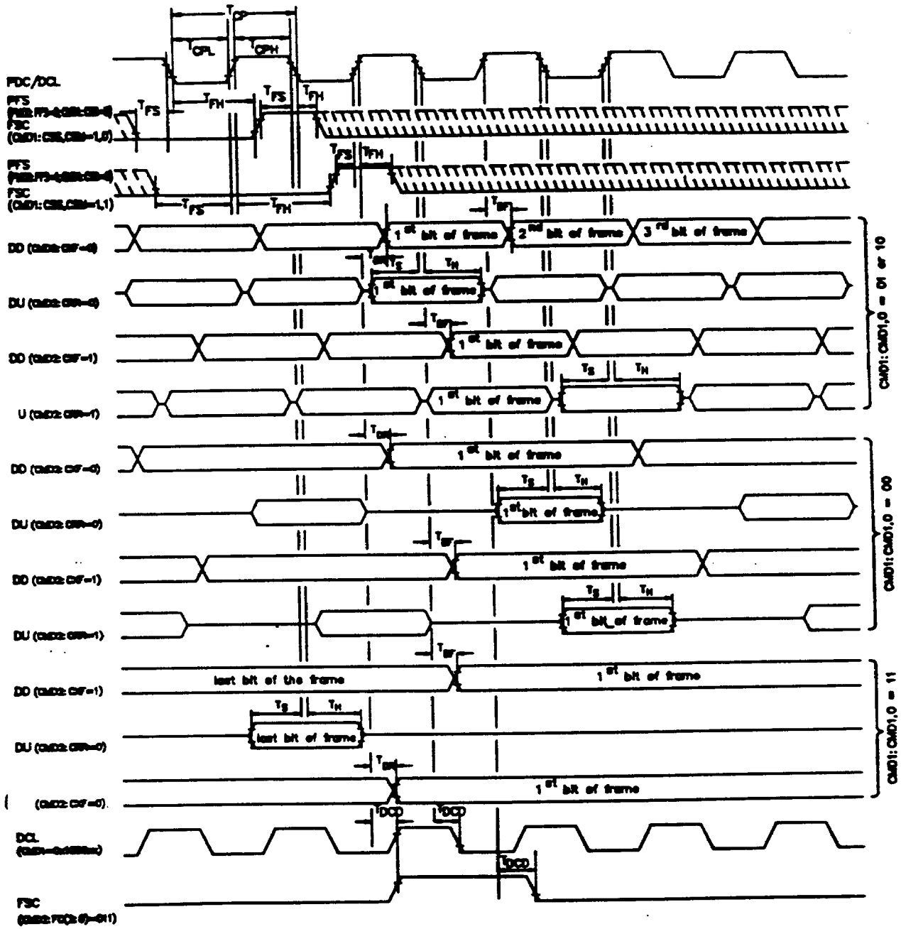
Fig. 5.9: AC Characteristics at the CFI with CMD:CSP1,0 = 10 (Prescaler Divisor = 1)
