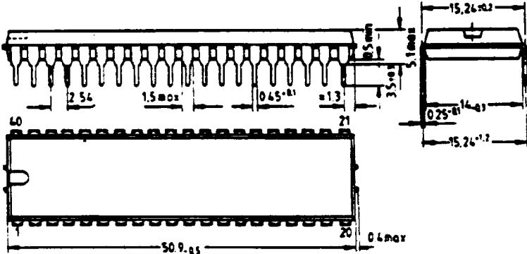
Fig. 5.14: Plastic Package, 40 Pins, P-DIP 40
