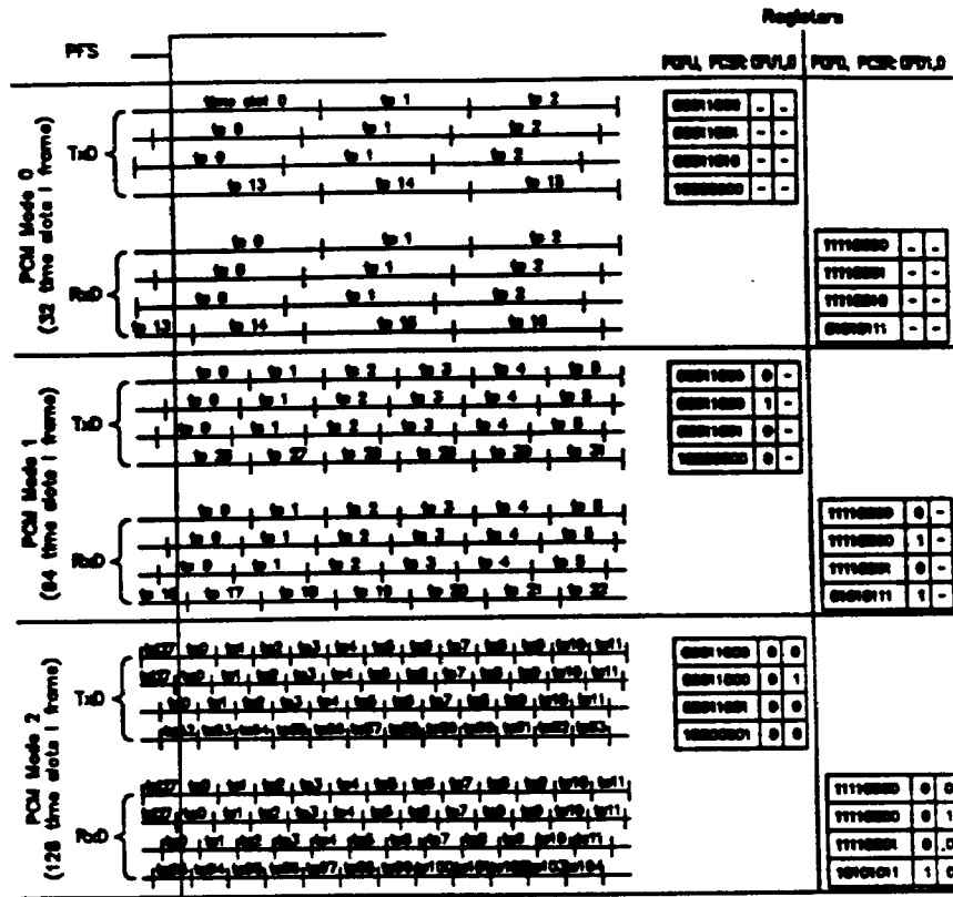
Fig. 4.2: PCM Interface Framing Offset
