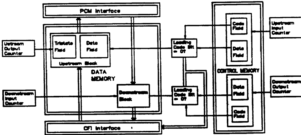
Figure 2.2: EPIC Memory Structure
