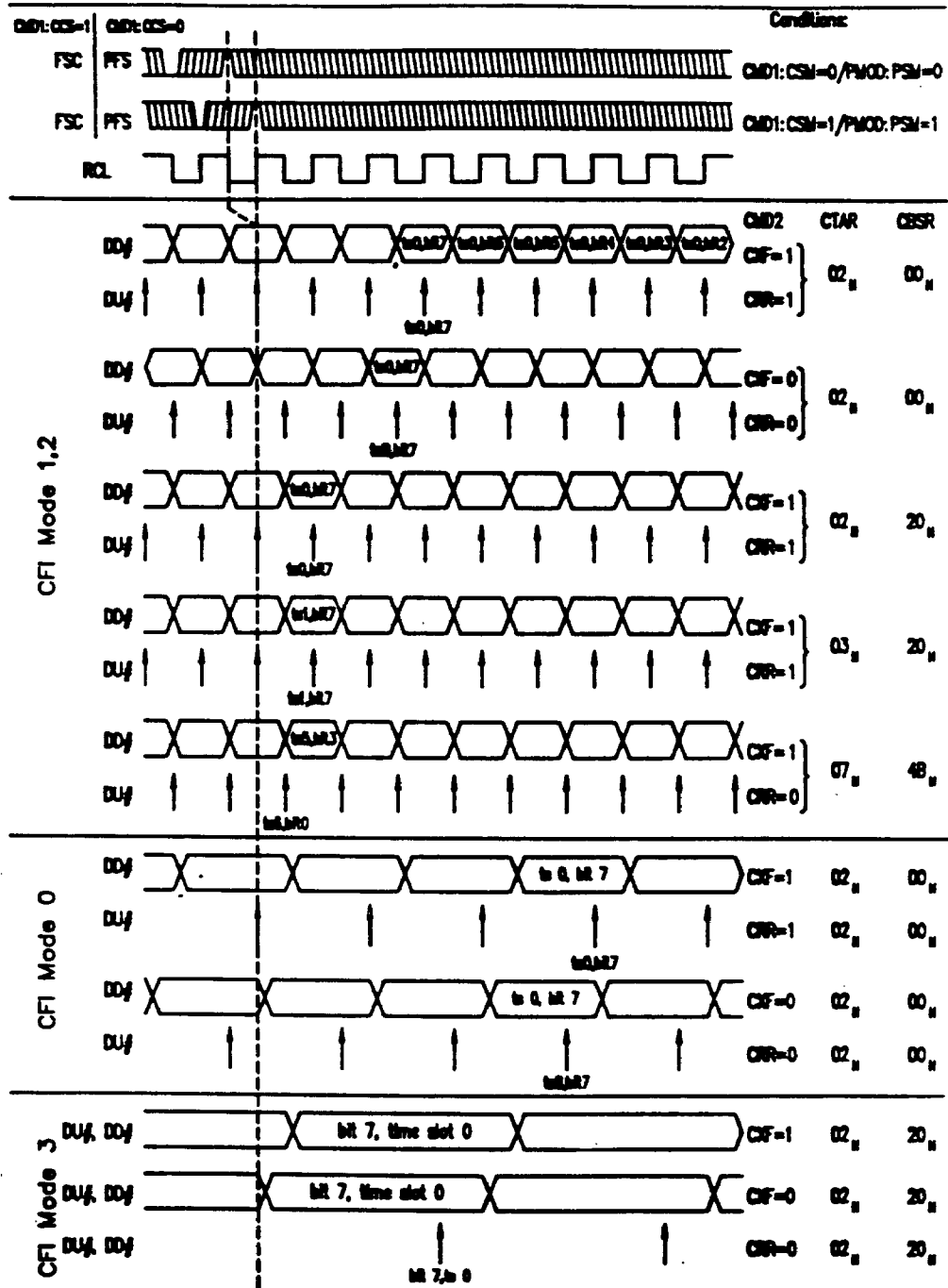
Fig. 4.6: Configurable Interface Bit Timing
