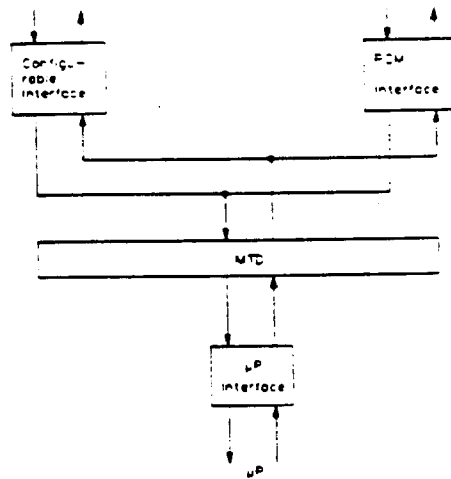
Figure 2.5: Synchron Transfer Paths between the μP, PCM and Configurable Interfaces
