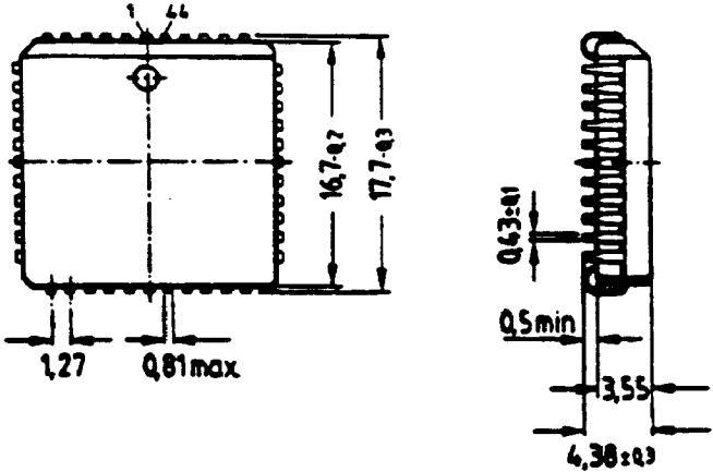
Fig. 5.15: Plastic Leadless Package, 44 Pins, PLCC 44
