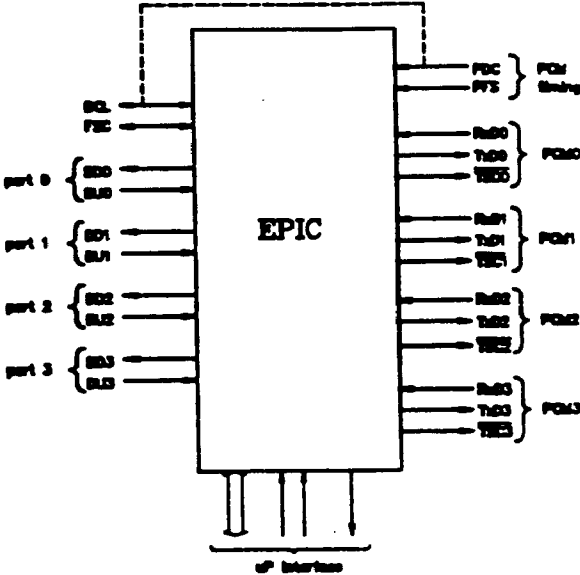
Fig. 1.2: Functional Symbol for the Duplex Configuration
