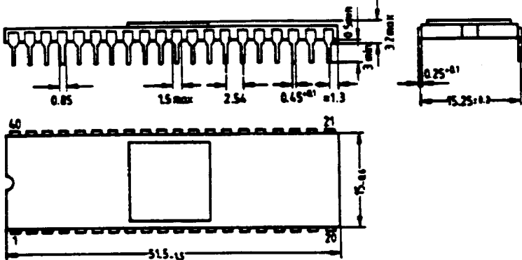
Fig. 5.13: Ceramic Package, 40 Pins, C-DIP 40
