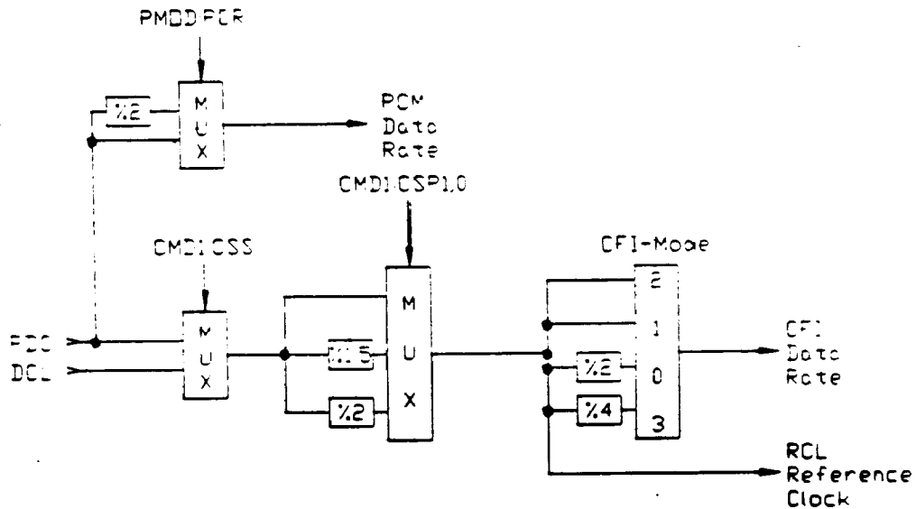
Figure 2.1: EPIC Clock Sources for the CFI and PCM Interface
