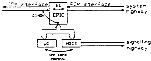
Fig. 1.7: Digital Line Card Architecture with a Completely Central D Channel Handling
