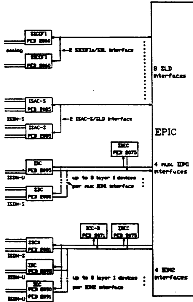
Fig. 1.4: Schematic Summary of the Line Card
