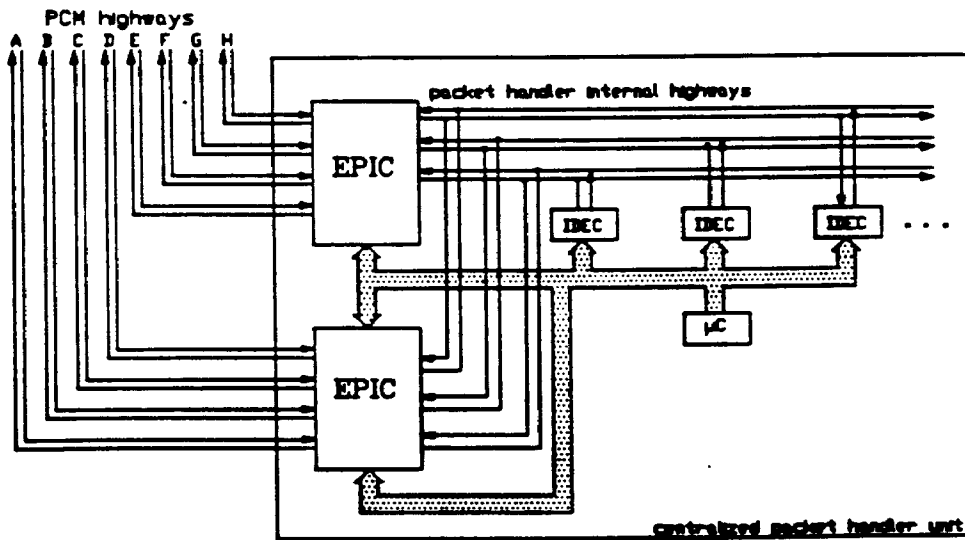
Fig. 1.12: Centralized Packet Handler with 3 Internal Highways
