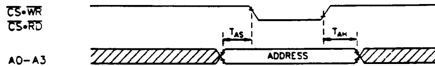
Fig. 5.4: Multiplexed Address Timing
