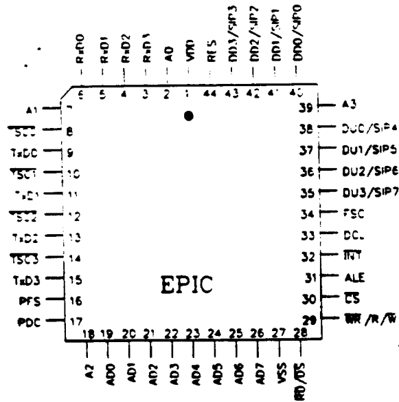
Fig. 1.1: Pin Configurations (top view)
