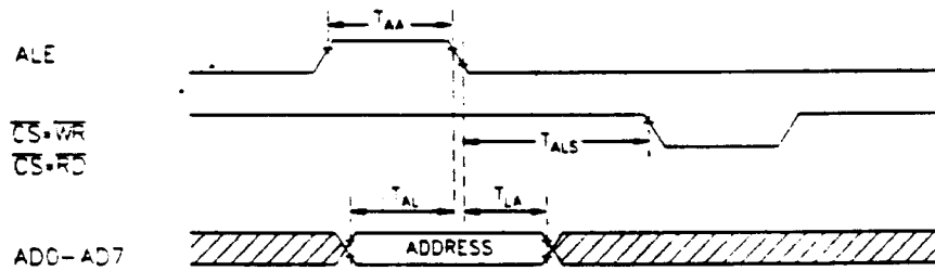
Fig. 5.4: Multiplexed Address Timing
