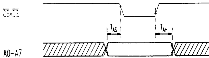
Fig. 5.8: Address Timing
