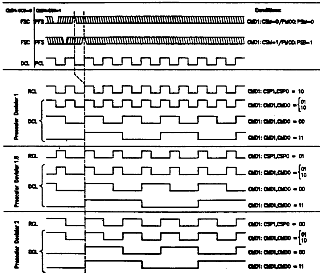
Fig. 4.5: Data Clock and Reference Clock for the different Prescaler Divisors at the CFI.
