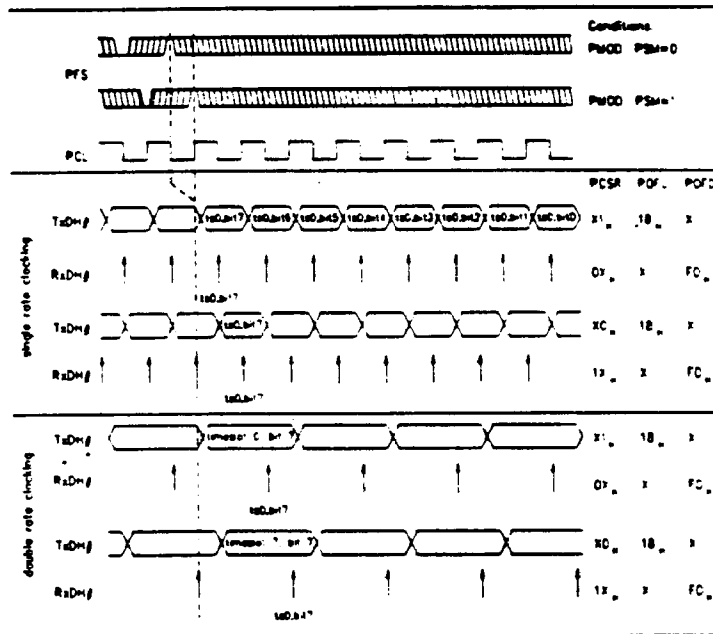
Fig. 4.1: Upstream and Downstream Timing at the PCM Interface for Single and Double Rate Clocking.
