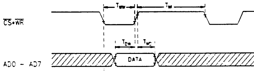
Fig. 5.3: \mu P Write Cycle
