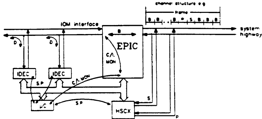
Fig. 1.6: Completely Decentral Packet Switching Digital Line Card Architecture
