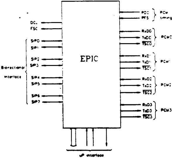
Fig. 1.3: Functional Symbol for the Bidirectional Configuration
