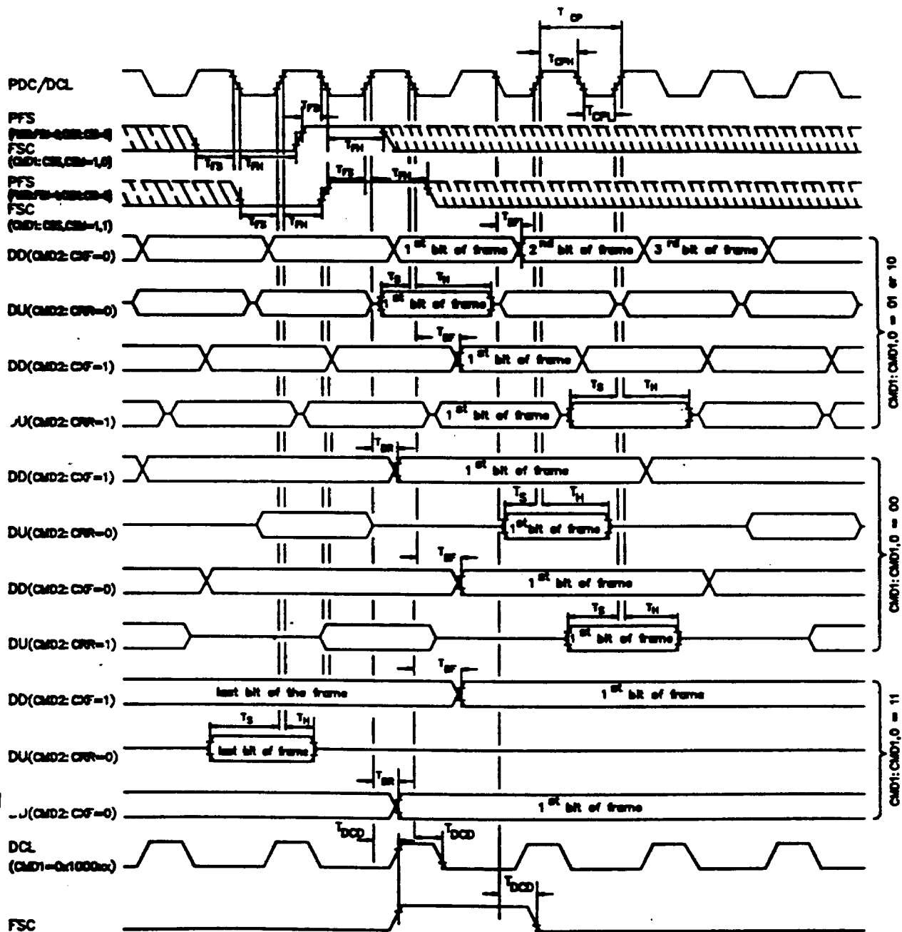
Fig. 5.10: AC Characteristics at the CFI with CMD1:CSP = 01 (Prescaler Divisor = 1.5)
