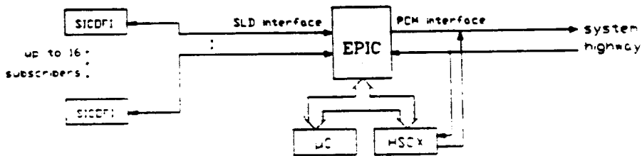
Fig. 1.5: Example of an Analog Line Card Architecture
