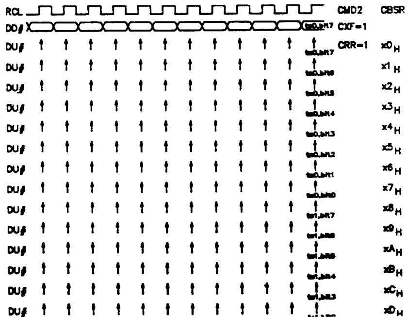
Fig.4.7.: CFI Upstream Bit Shifting
