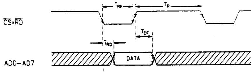
Fig. 5.2: \mu P Read Cycle
