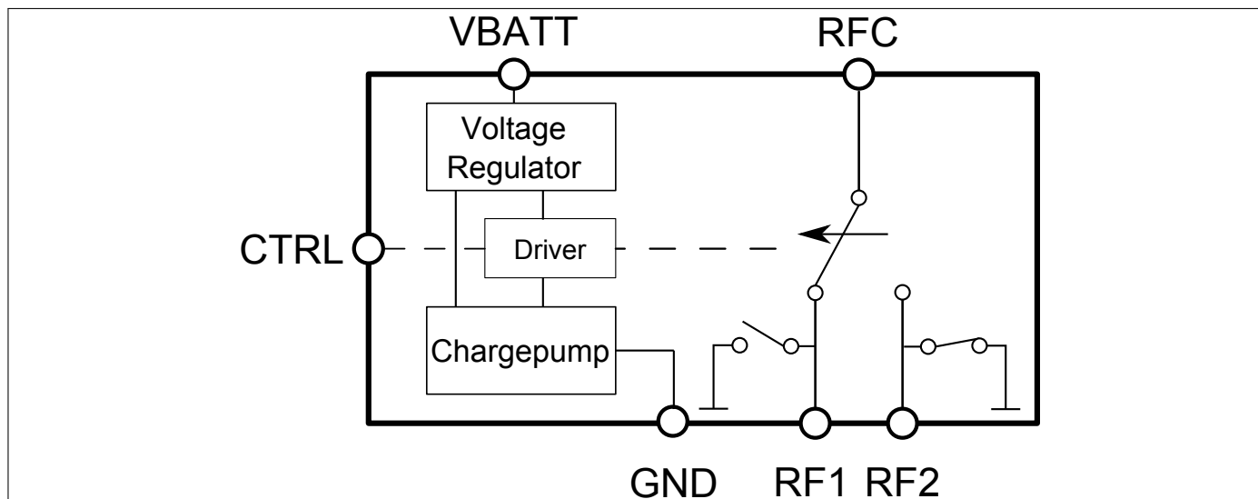
Figure 1: BGS12PN10 block diagram
