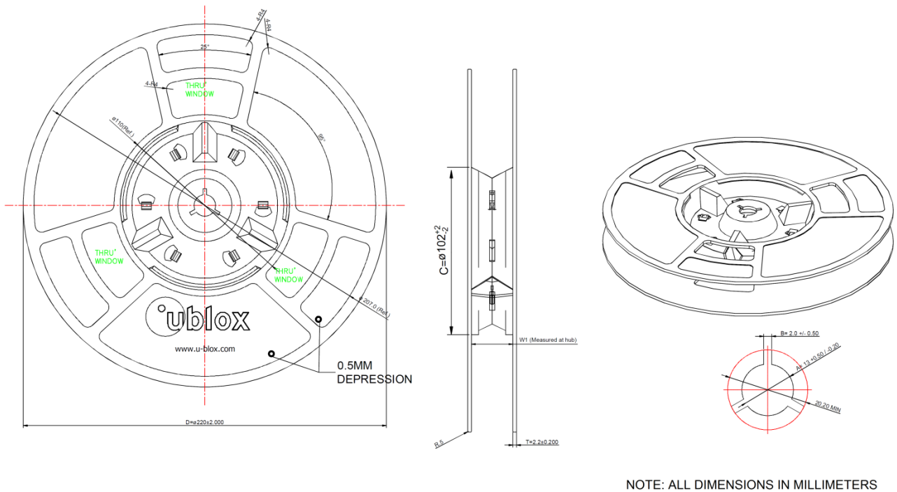
Figure 4: SARA-R4 series modules reel
