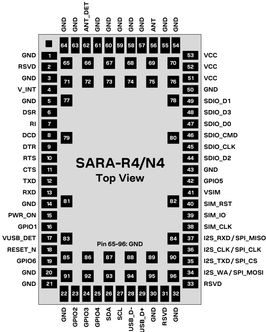
Figure 2: SARA-R4 series pin assignment (top view)
