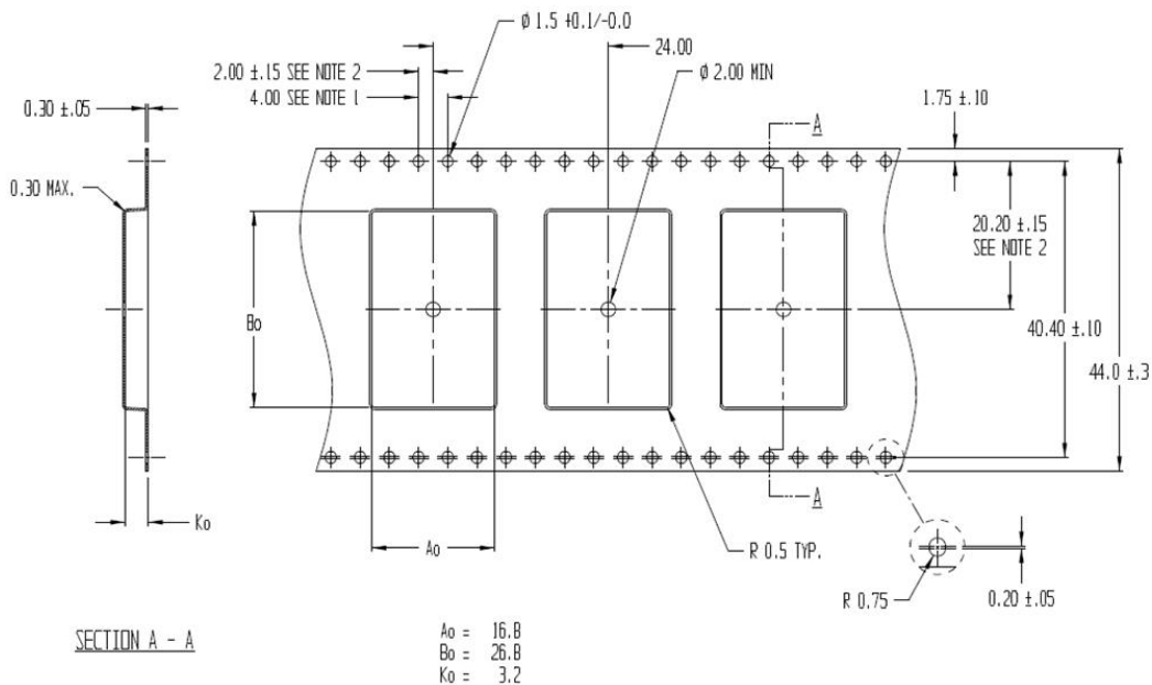
Figure 6: SARA-R4 series modules tape
