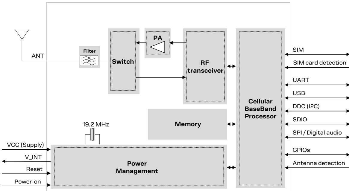
Figure 1: SARA-R4 series block diagram
