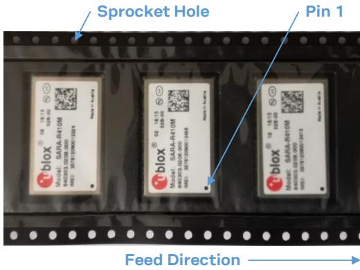
Figure 5: Orientation of SARA-R4 series modules on tape
