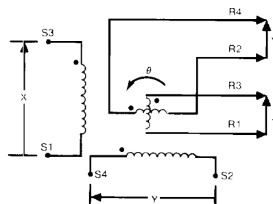
FIGURE 11 Computing Resolver Schematic
