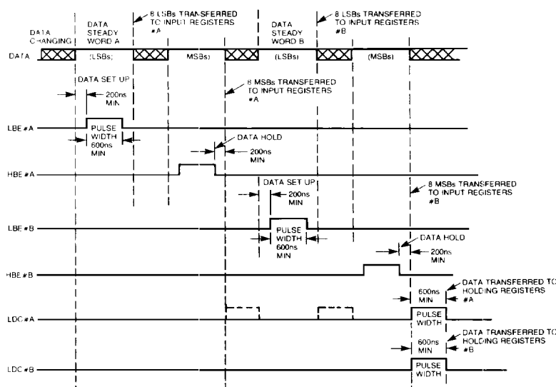
FIGURE 7 Two-Byte Loading.
