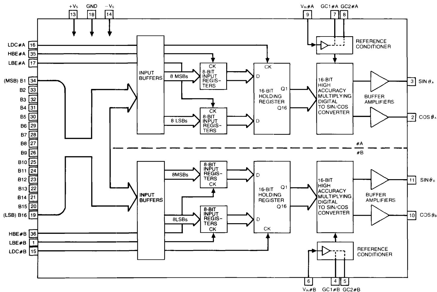
FIGURE 1 2036 BLOCK DIAGRAM
