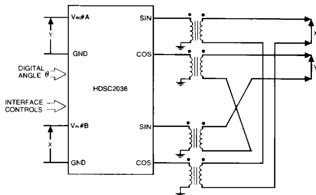
FIGURE 10 HDSC2036 Connected as Computing Resolver
