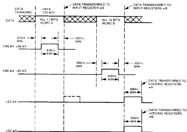
FIGURE 9 Single-Byte Loading.
